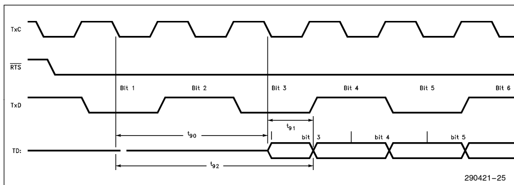
Figure 26. TPE Transmit Timings (Start of Frame)
