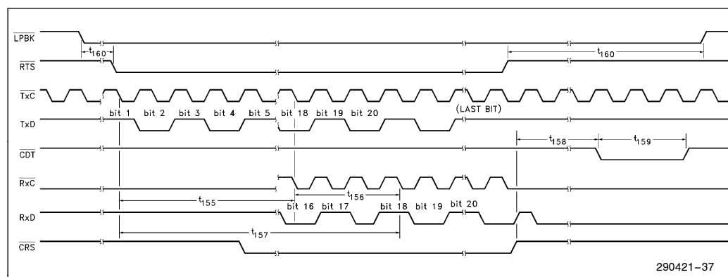
Figure 38. Loopback Timings
