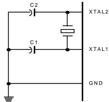
Figure 1. Oscillator Connections
