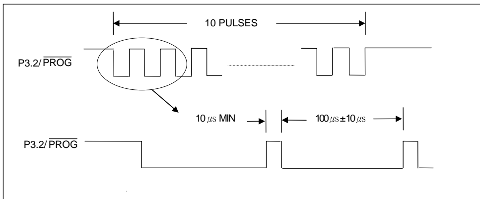
Figure 8. Programming Waveform
