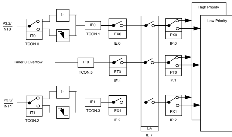
Figure 4. Interrupt Request Sources
