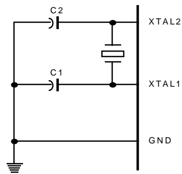
Figure 1. Oscillator Connections
