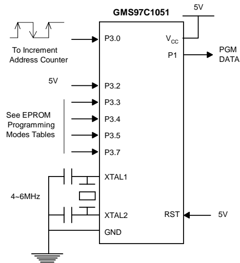
Figure 6. Verifying the EPROM Memory
