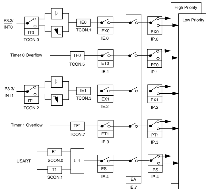
Figure 4. Interrupt Request Sources
