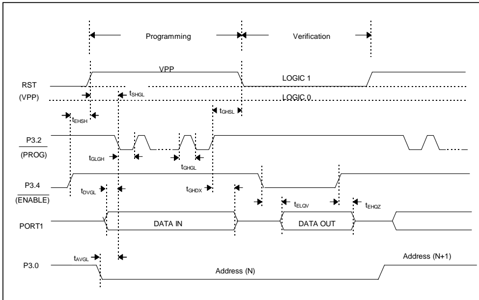
Figure 7. EPROM Programming and Verification
