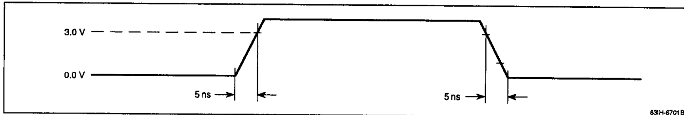
Figure 1. Input Timing
