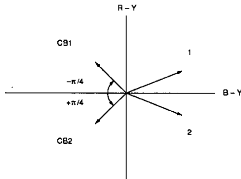
Figure 3. Background color-phase vector diagram
