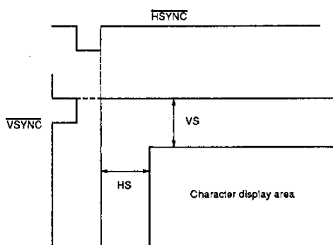
Figure 2. Vertical and horizontal sync pulses
