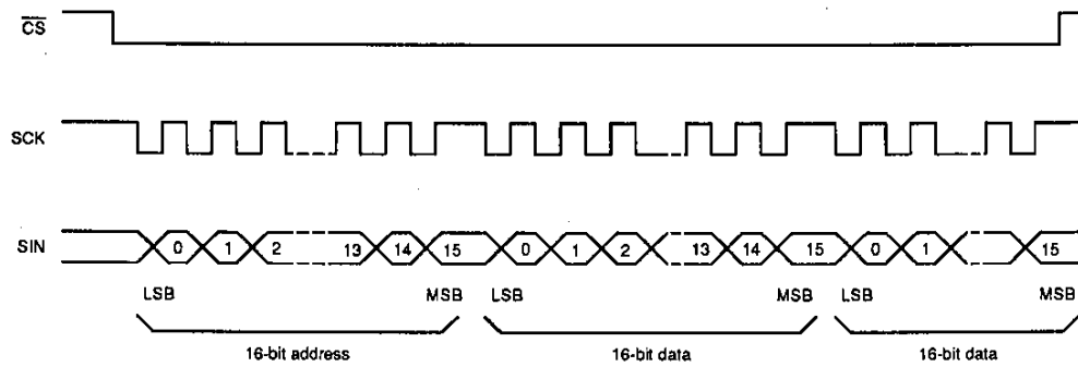
Figure 1. Input timing
