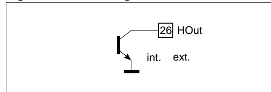
Figure 9. HOut configuration
