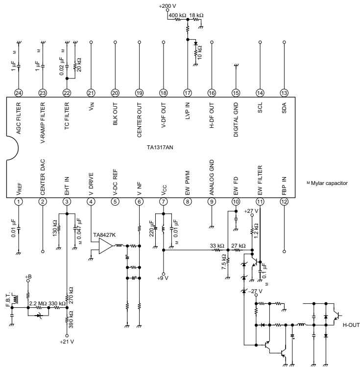
Application Circuit 1 (V-AC coupling/EW parabola output)
