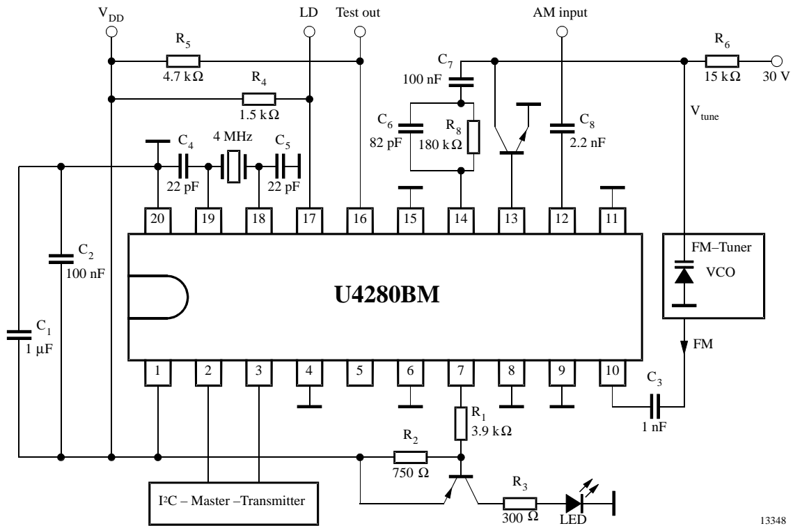
Figure 7. Application circuit
