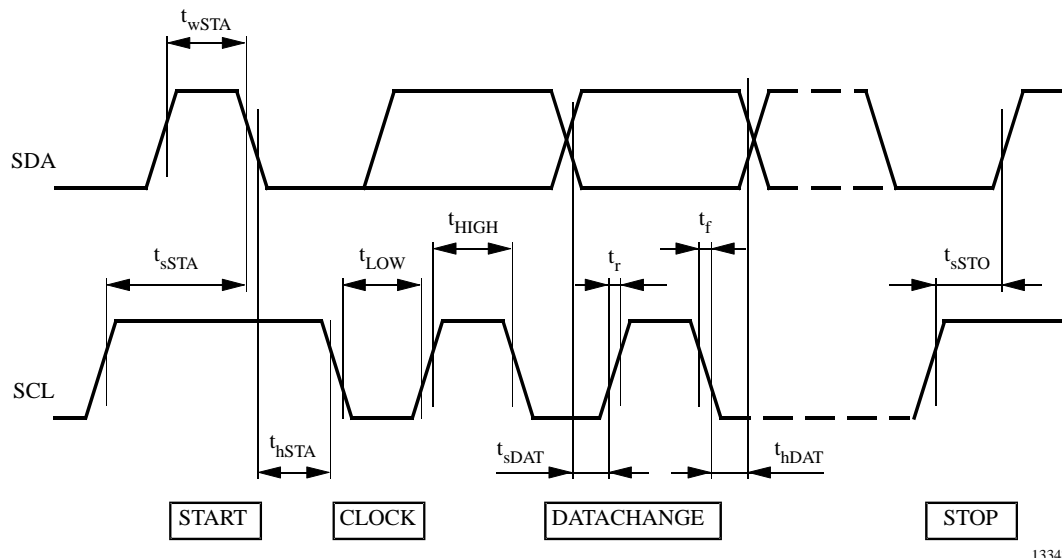
Figure 5. Bus timing
