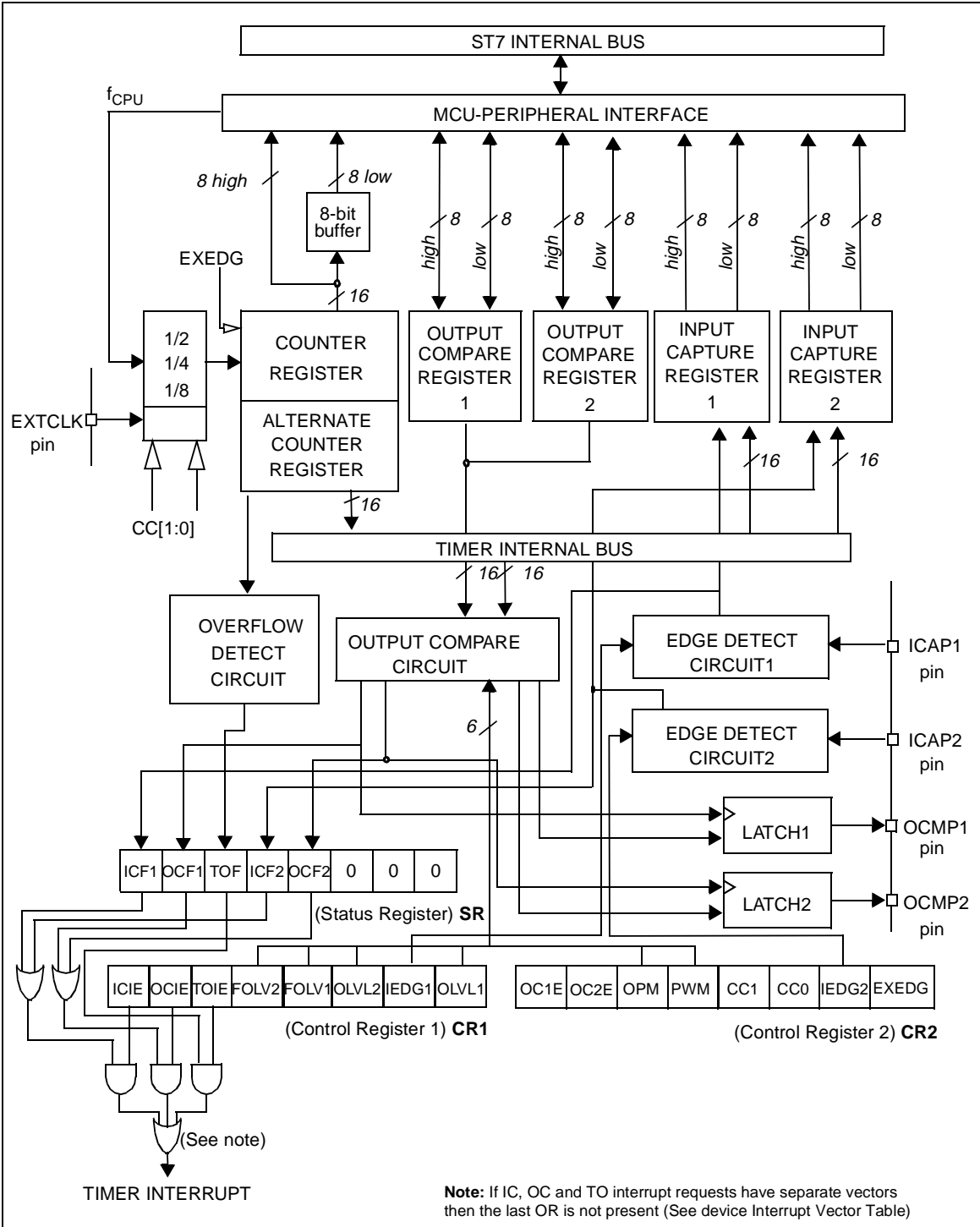
Figure 18. Timer Block Diagram
