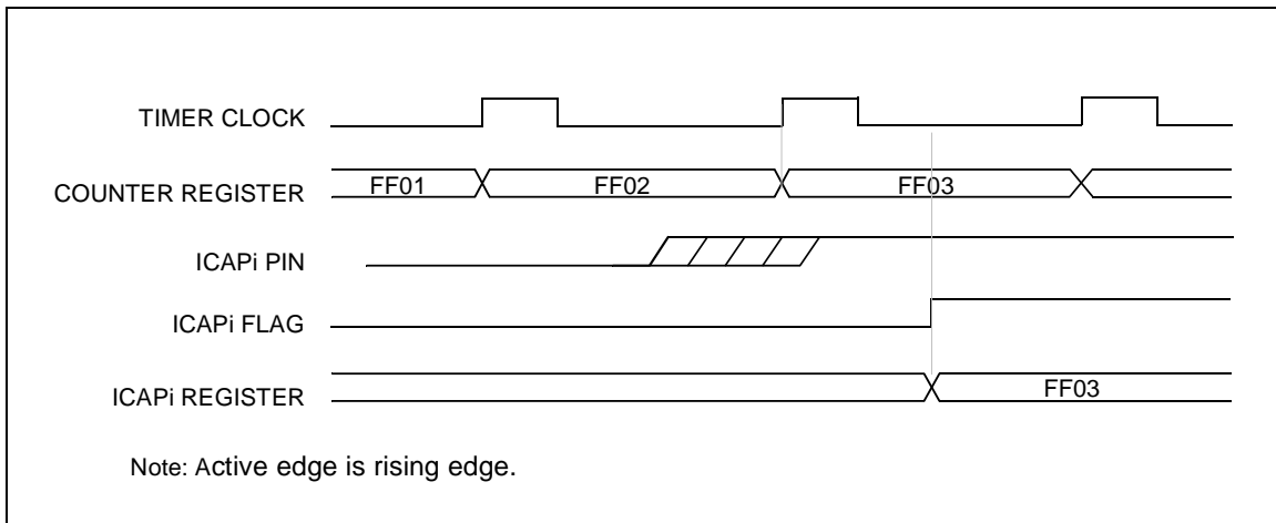
Figure 23. Input Capture Timing Diagram
