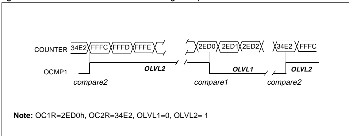
Figure 28. Pulse Width Modulation Mode Timing Example
