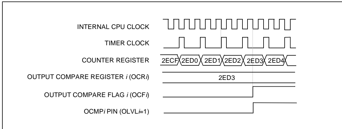
Figure 25. Output Compare Timing Diagram, f_{\text{TIMER}} = f_{\text{CPU}}/2
