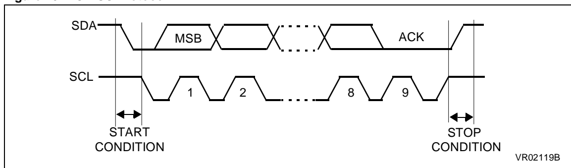
Figure 29. I 2 C BUS Protocol
