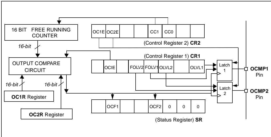
Figure 24. Output Compare Block Diagram
