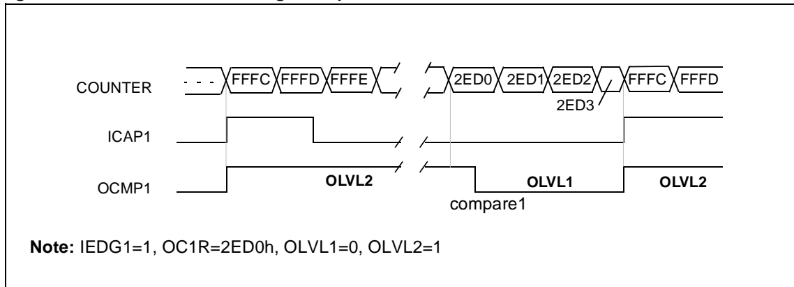
Figure 27. One Pulse Mode Timing Example
