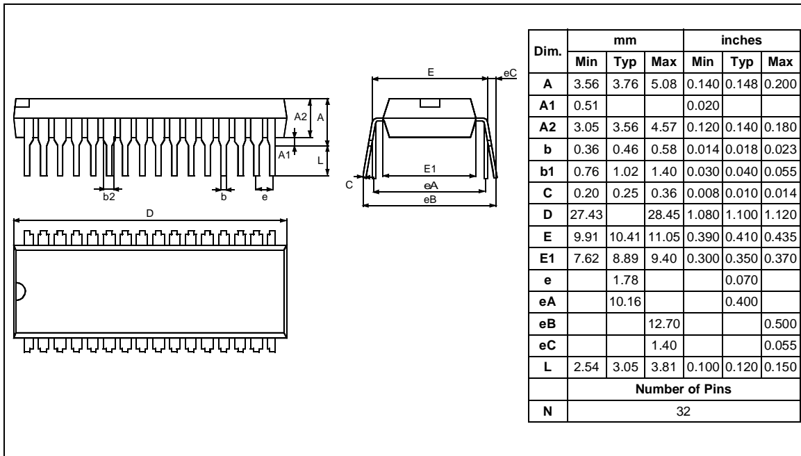
Figure 53. 32-Pin Shrink Ceramic Dual In-Line Package
