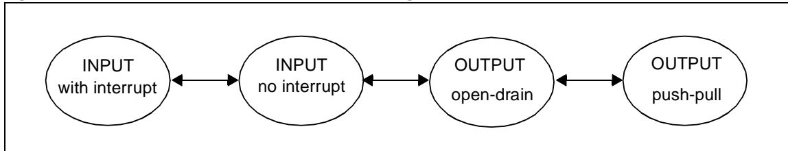
Figure 15. Recommended I/O State Transition Diagram
