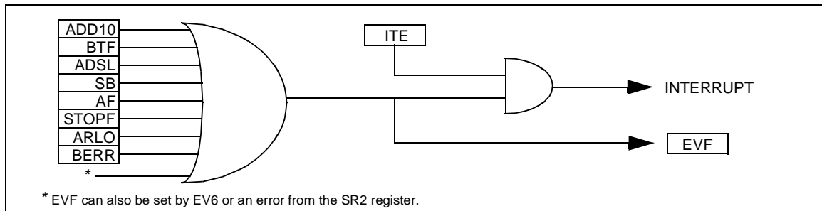
Figure 32. Event Flags and Interrupt Generation
