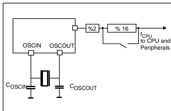
Figure 10. Clock Prescaler Block Diagram
