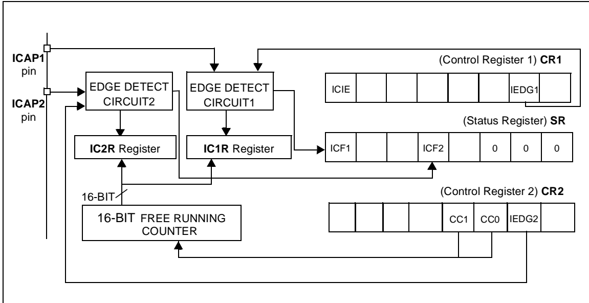
Figure 22. Input Capture Block Diagram
