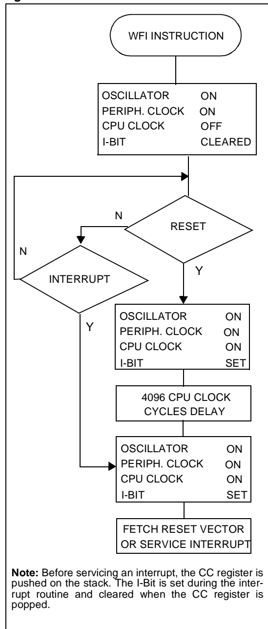
Figure 13. WAIT Flow Chart
