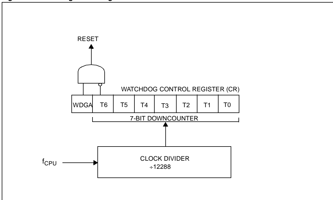
Figure 17. Watchdog Block Diagram
