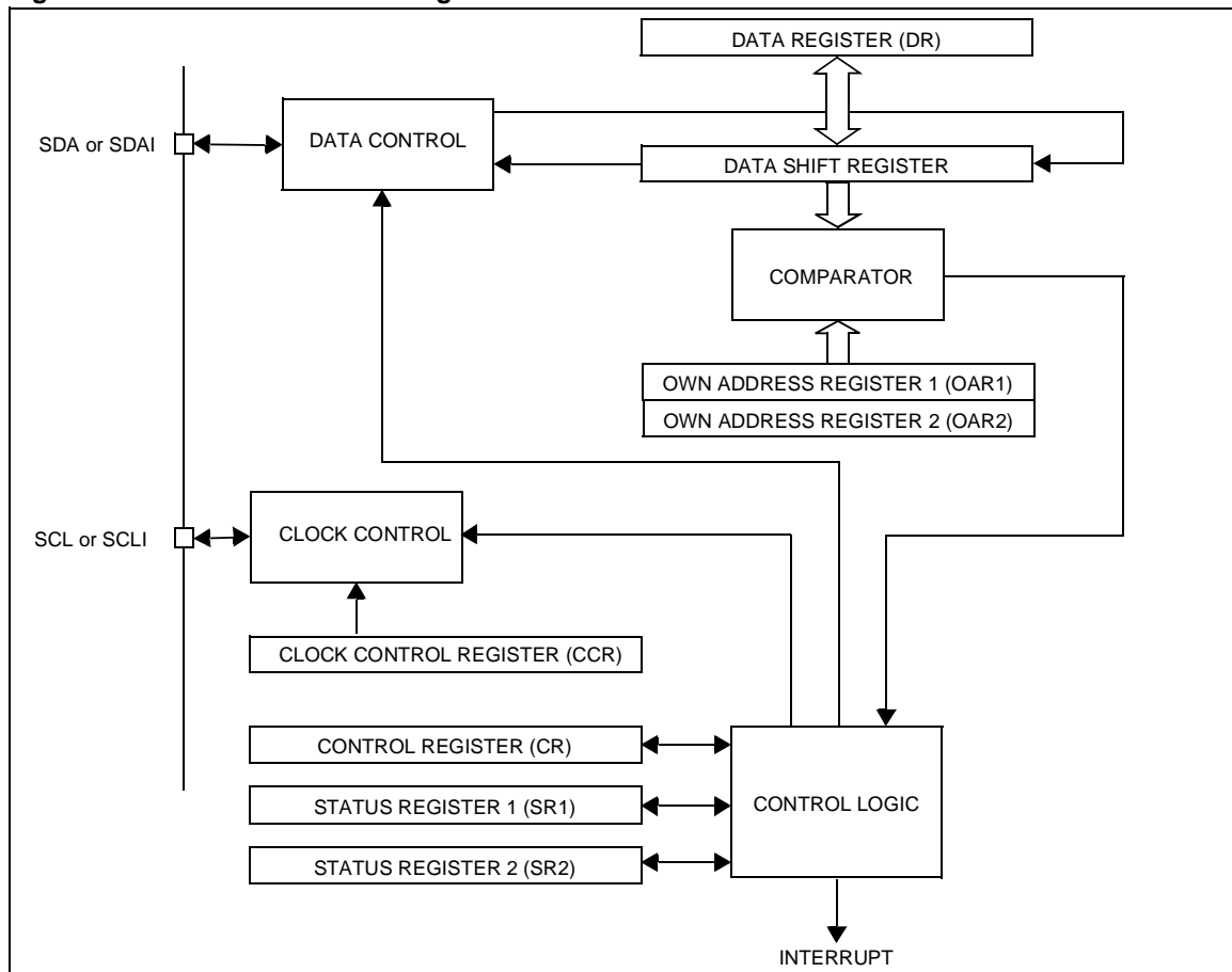
Figure 30. I 2 C Interface Block Diagram
