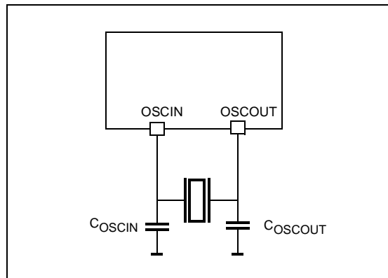
Figure 9. Crystal/Ceramic Resonator
