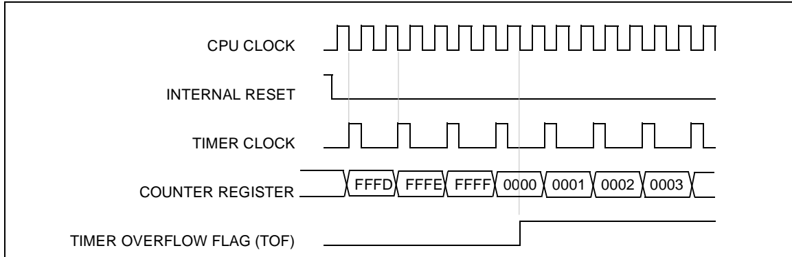
Figure 19. Counter Timing Diagram, internal clock divided by 2
