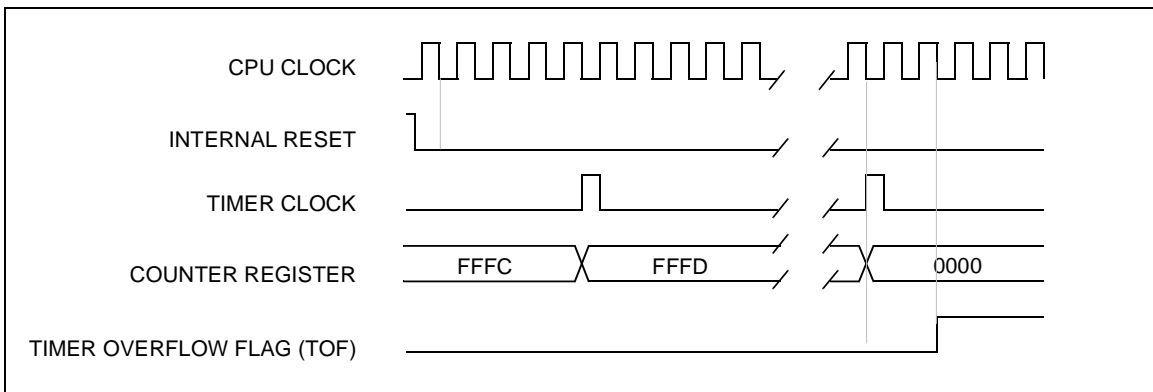
Figure 21. Counter Timing Diagram, internal clock divided by 8
