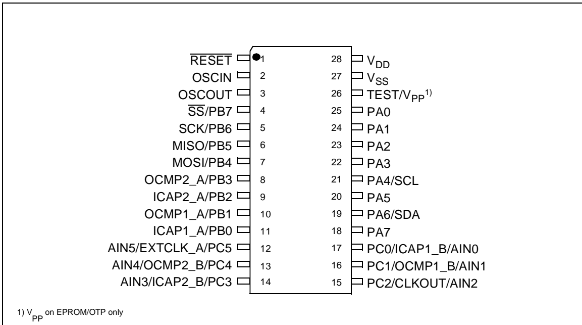
Figure 3. ST72251 Pinout (SO28)
