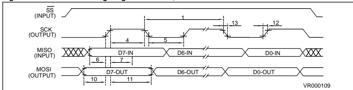
Figure 43. SPI Master Timing Diagram \text{CPHA}=0 , \text{CPOL}=0
