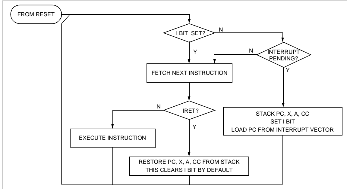
Figure 12. Interrupt Processing Flowchart
