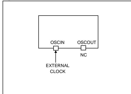
Figure 8. External Clock Source Connections
