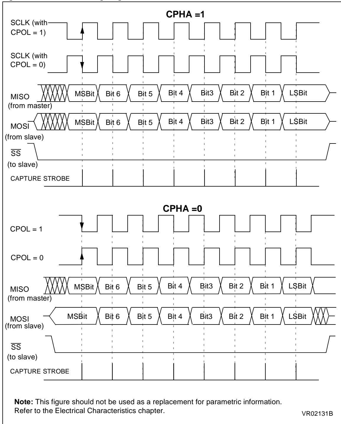
Figure 36. Data Clock Timing Diagram
