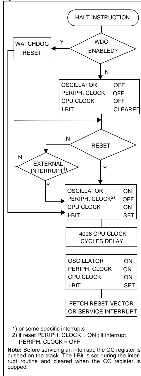
Figure 14. HALT Flow Chart
