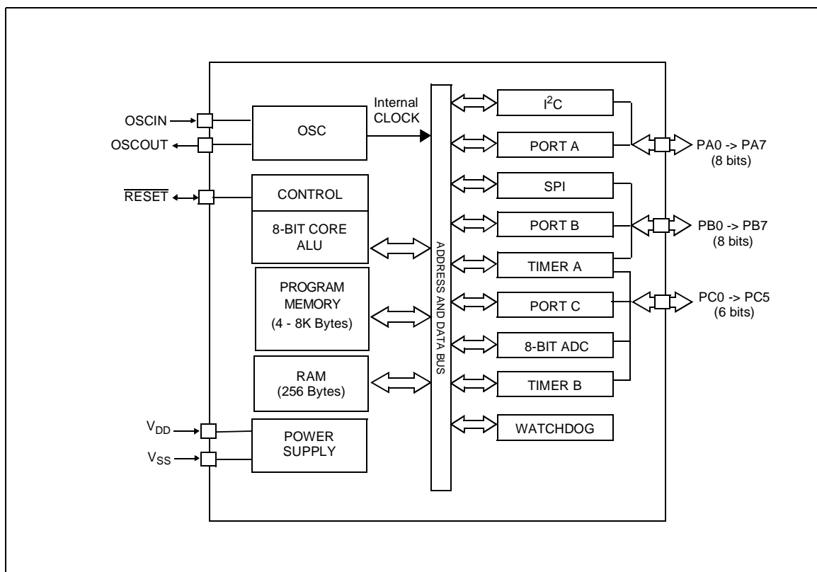
Figure 1. ST72251 Block Diagram
