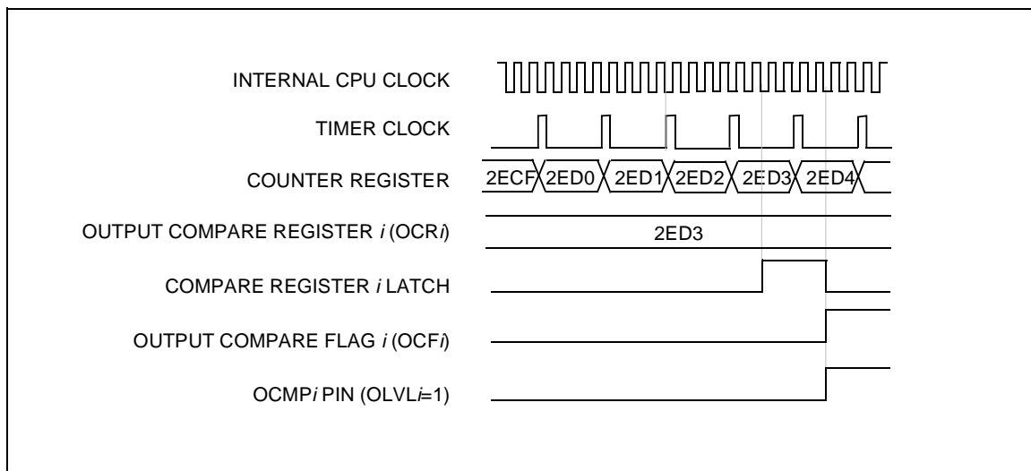
Figure 26. Output Compare Timing Diagram, f_{\text{TIMER}} = f_{\text{CPU}}/4
