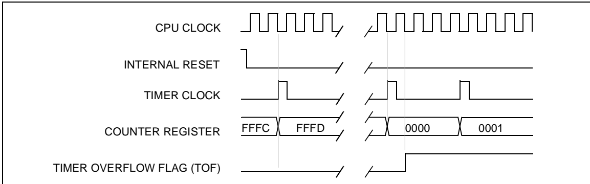
Figure 20. Counter Timing Diagram, internal clock divided by 4
