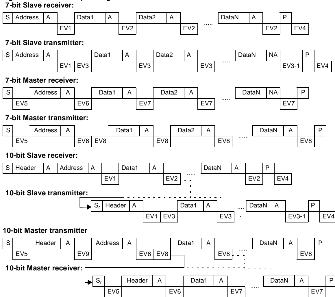
Figure 31. Transfer Sequencing
