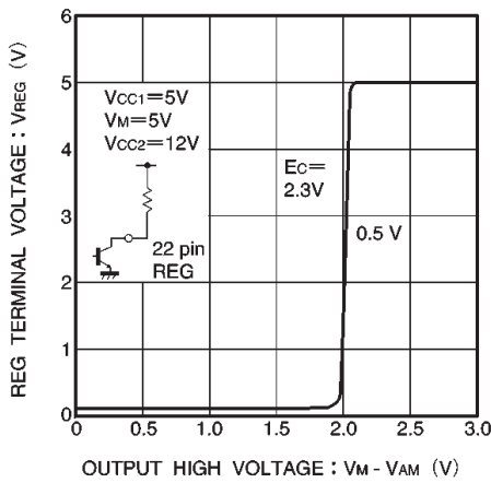
Fig.15 REG-pin voltage vs. output high level voltage
