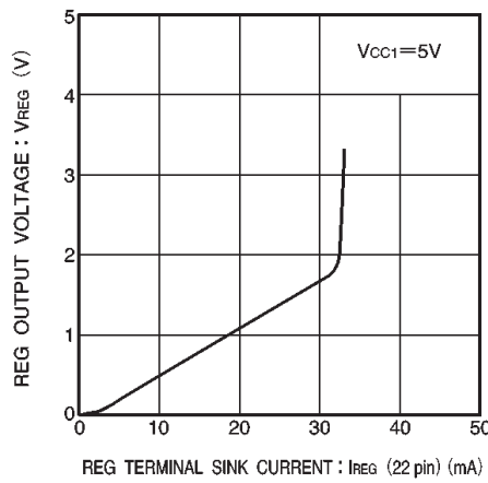
Fig.16 REG-pin output voltage vs. REG-pin sink current
