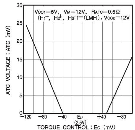
Fig.11 Output current vs. torque control voltage ( III )
