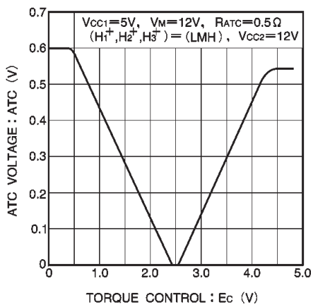
Fig.9 Output current vs. torque control voltage ( I )
