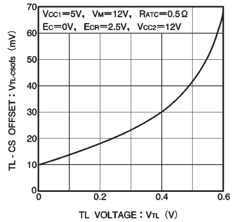
Fig.14 TL-CS offset vs. TL voltage
