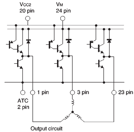
Fig.4 Output circuit
