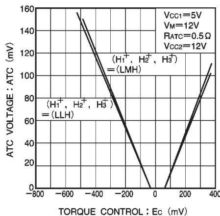
Fig.10 Output current vs. torque control voltage ( II )
