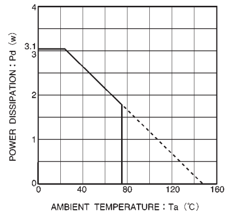
Fig.17 Power dissipation curve
