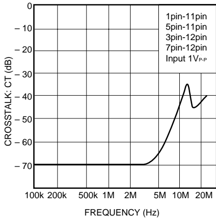
Fig. 16 Crosstalk characteristic (OUT2 and OUT3)
