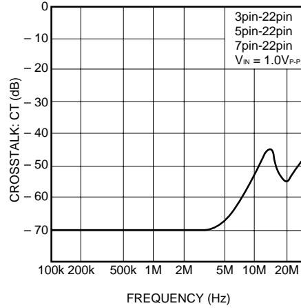
Fig. 14 Crosstalk characteristic (OUT1)
