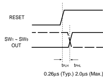
Fig. 8 Reset and output relationship (reset transmission time)
