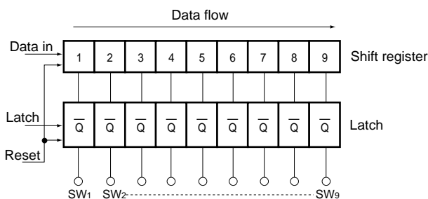
Fig. 5 Digital block
