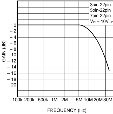
Fig. 13 Frequency characteristic(OUT1)
