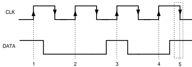
At points 1 to 4 data is input to the shift register. At point 5 the contents of the shift register are transferred to the latch and simultaneously output.
