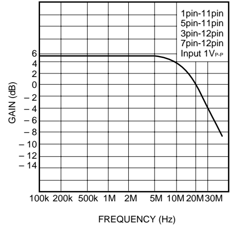
Fig. 15 Frequency characteristic (OUT2 and OUT3)
