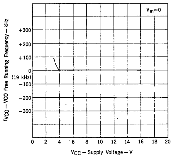
VCO FREE RUNNING FREQUENCY vs. SUPPLY VOLTAGE
