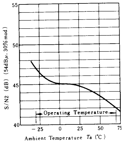
SIGNAL-TO-NOISE RATIO vs. AMBIENT TEMPERATURE
