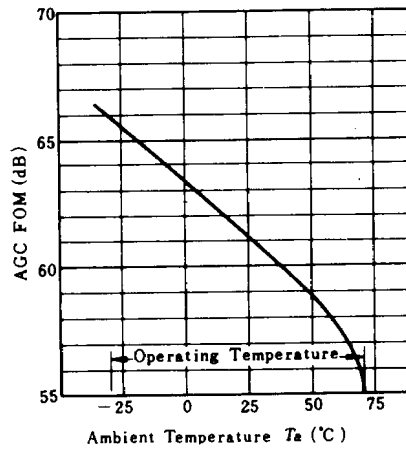
AGC FOM vs. AMBIENT TEMPERATURE
