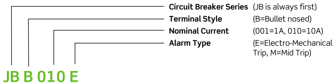
Figure 11 - Circuit Breaker Naming Convention
