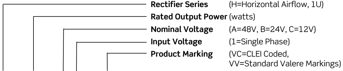
Figure 3 - H Series Rectifiers Numbering Convention
