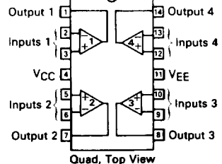
P SUFFIX PLASTIC PACKAGE CASE 646
