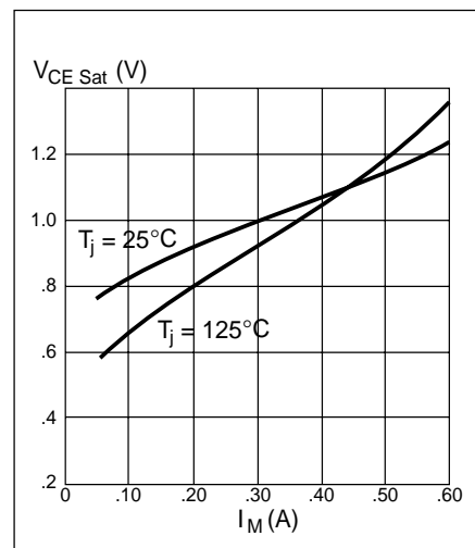
Figure 9. Typical source saturation voltage vs. output current.
