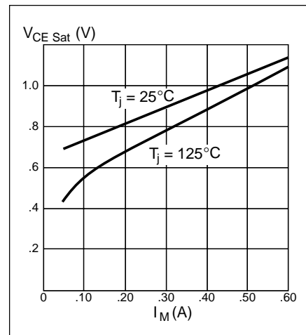
Figure 11 Typical sink saturation voltage vs. output current.
