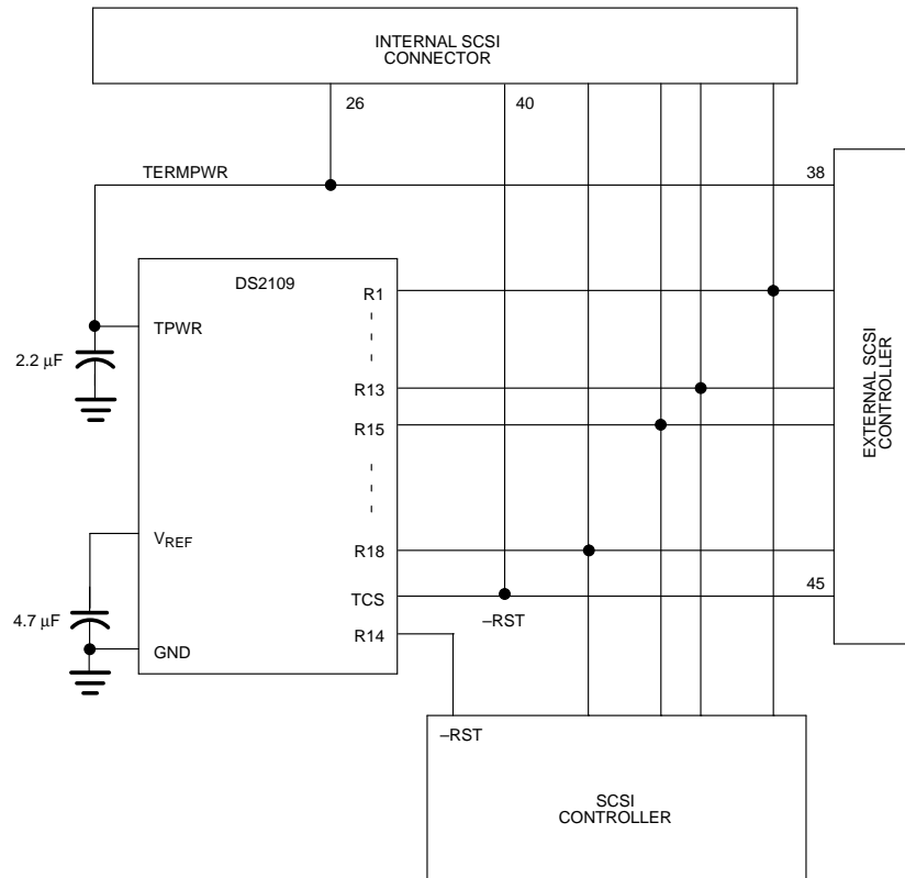
BUS CURRENT SENSE CONFIGURATION Figure 6
