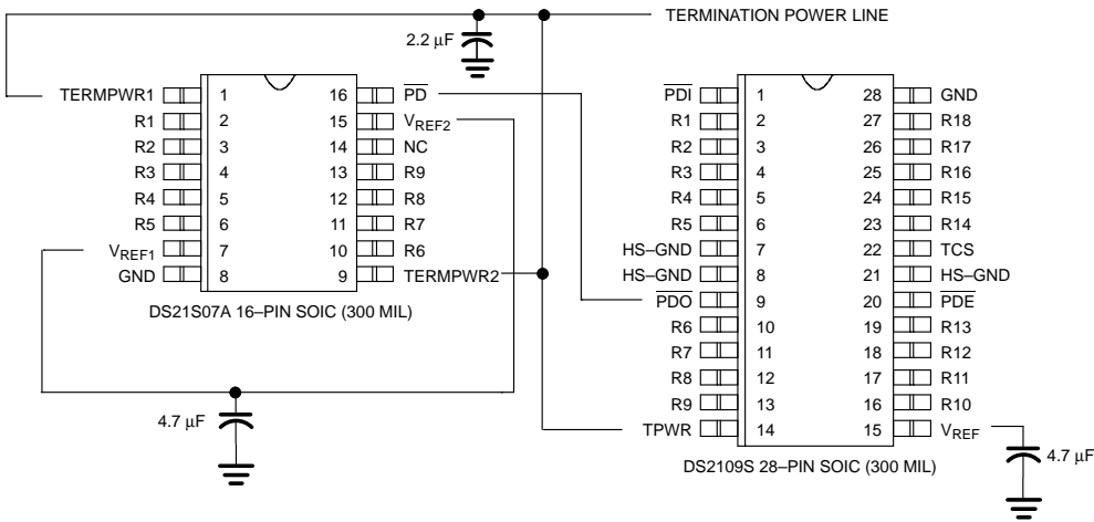
WIDE SCSI CONFIGURATION Figure 8
