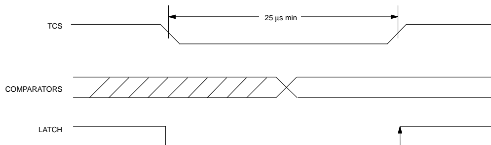
BUS CURRENT SENSE TIMING DIAGRAM Figure 7
