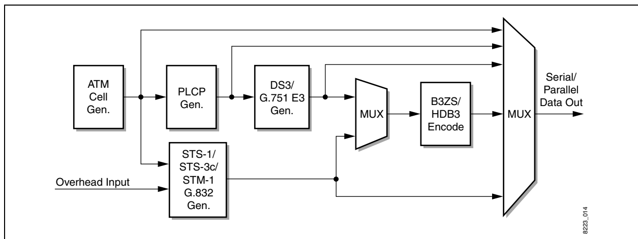
Figure 2-2. CN8223 Transmitter Block Diagram
