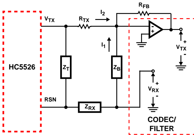
FIGURE 17. TRANSHYBRID CIRCUIT
