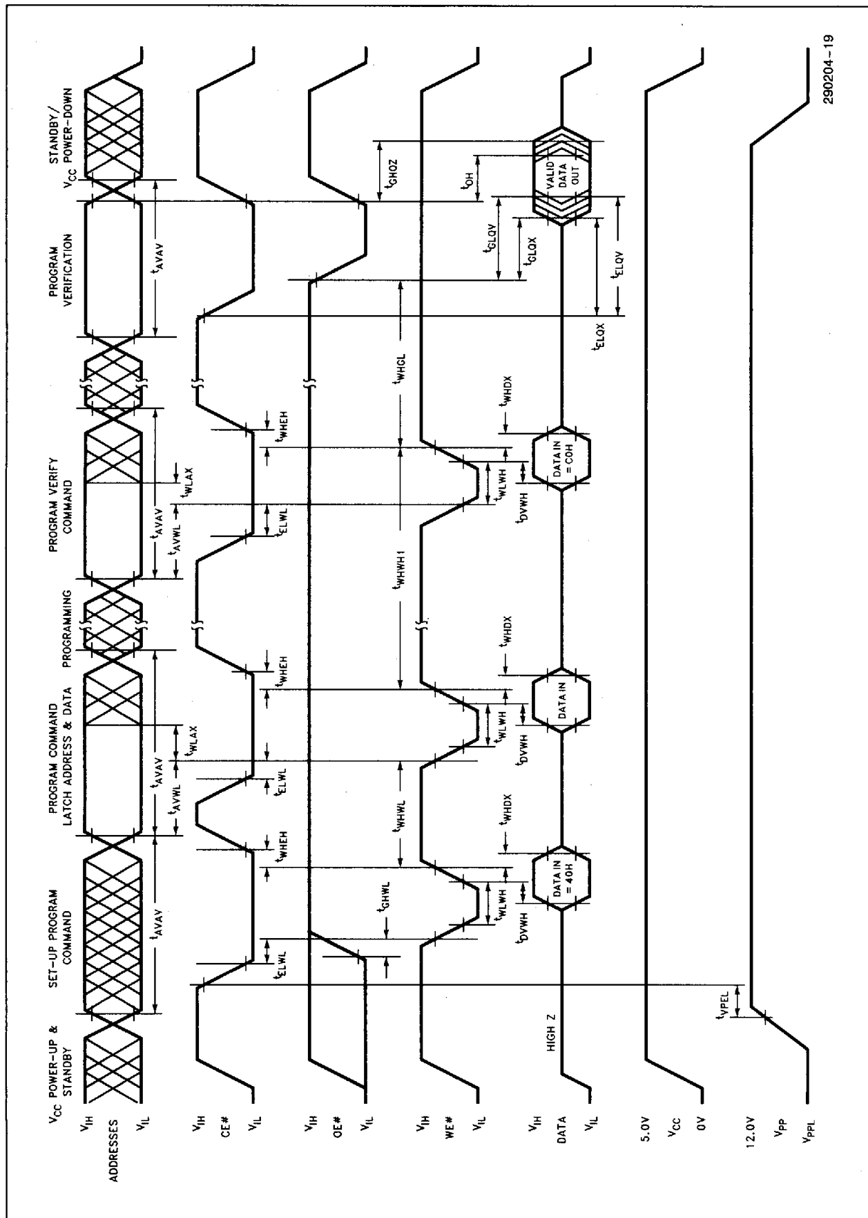
Figure 11. AC Waveforms for Programming Operations
