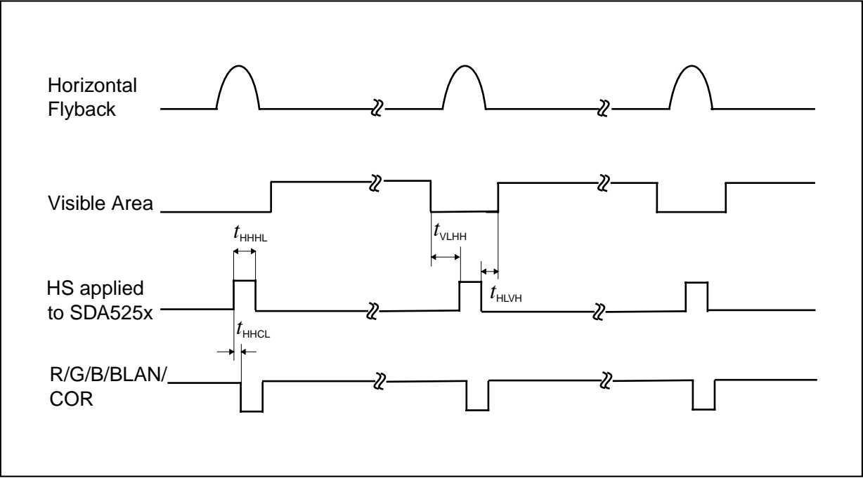
Figure 42 Horizontal Sync-Timing
