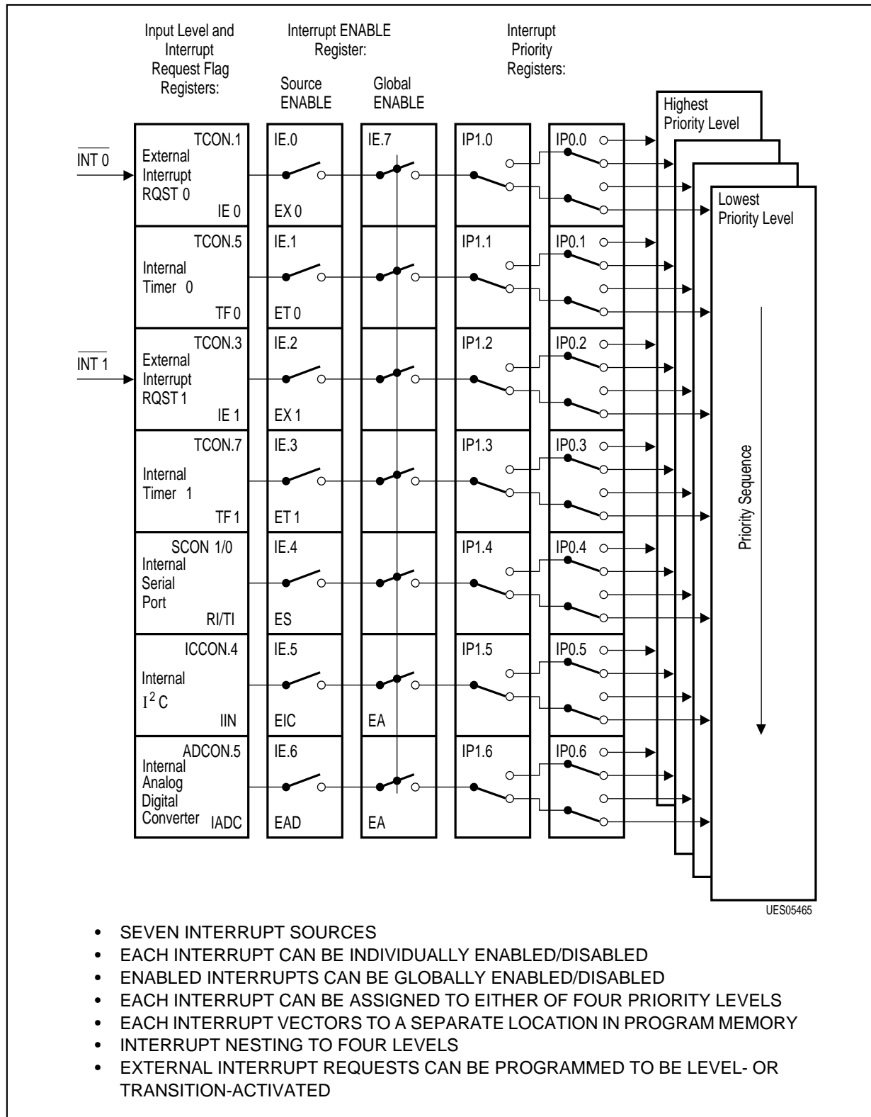
Figure 23 Interrupt System
