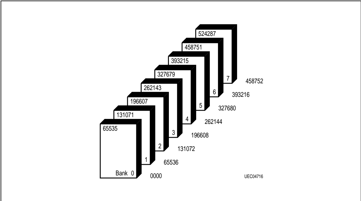
Figure 16 Bank Organization
