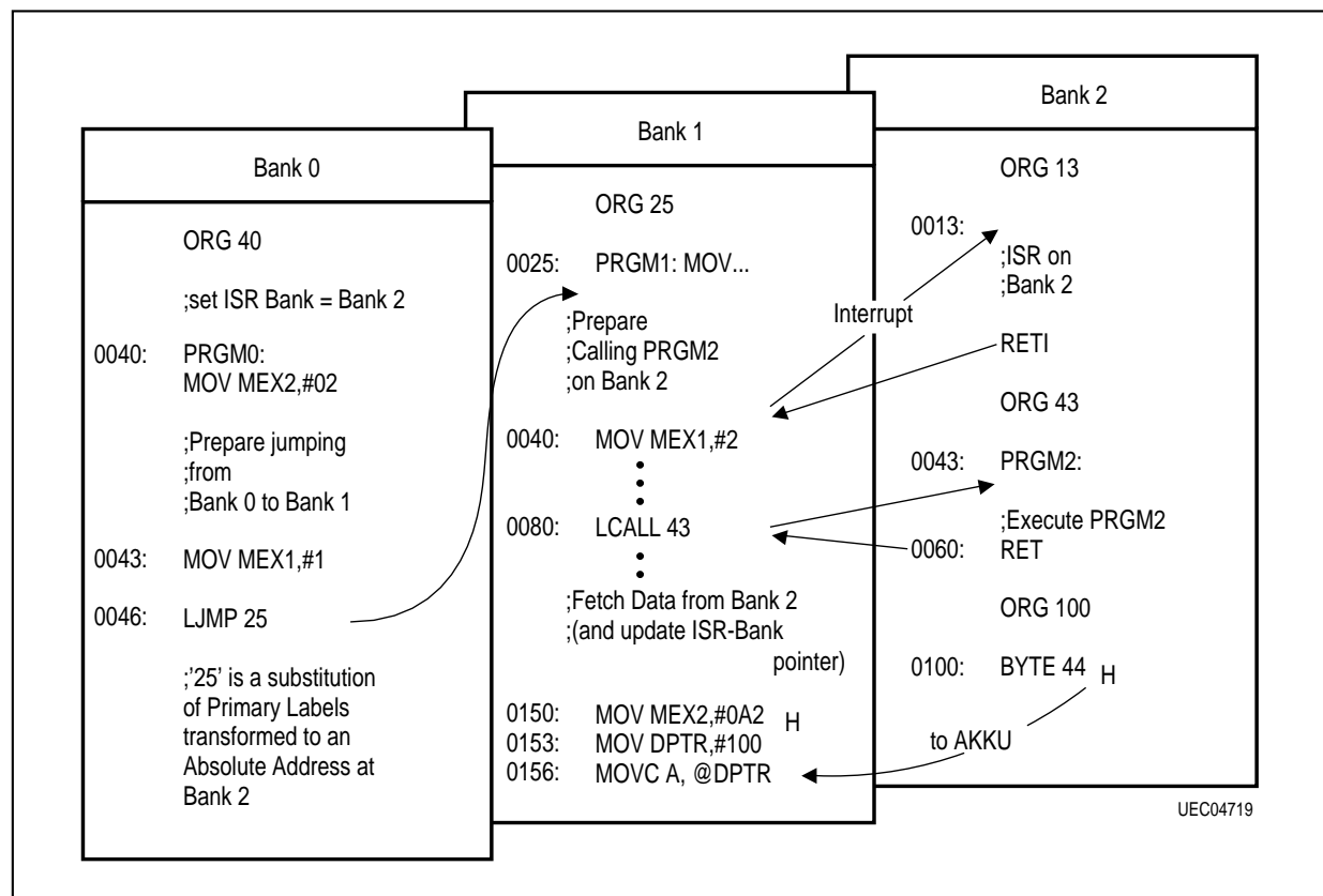
Figure 20 Program Example
