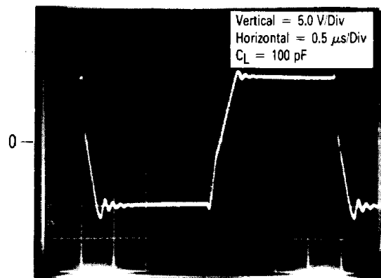
FIGURE 27 — LARGE-SIGNAL
