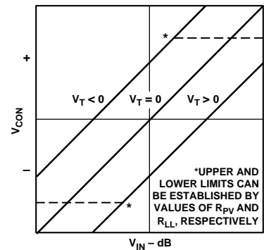
b. Typical Compandor Control Curves
