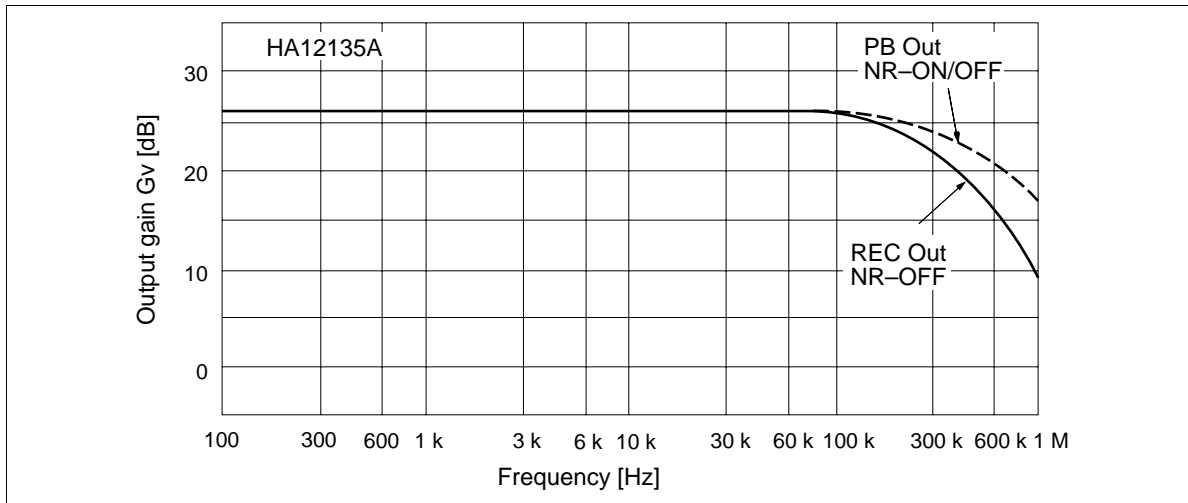
Figure 16 REC Mode Output Gain vs. Frequency
