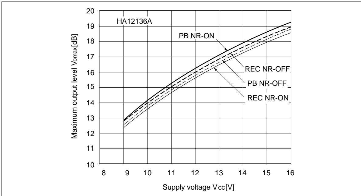
Figure 13 Maximum Output Level vs. Supply Voltage
