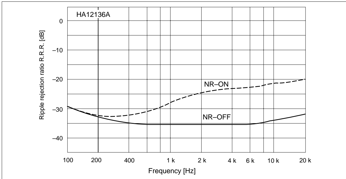
Figure 7 REC Mode Ripple Rejection Ratio vs. Frequency
