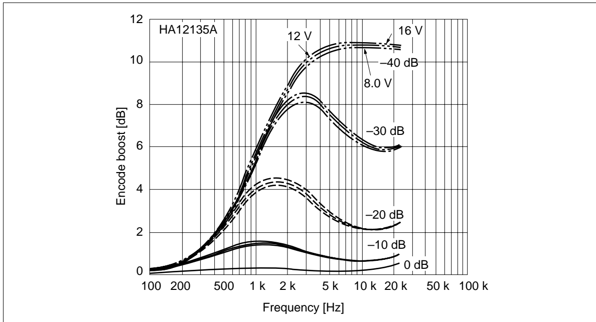
Figure 15 Encode Boost vs. Frequency
