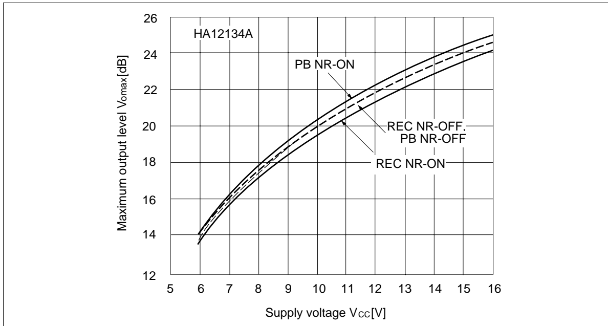
Figure 35 Maximum Output Level vs. Supply Voltage
