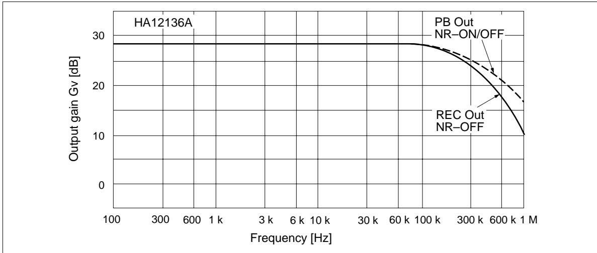
Figure 5 REC Mode Output Gain vs. Frequency
