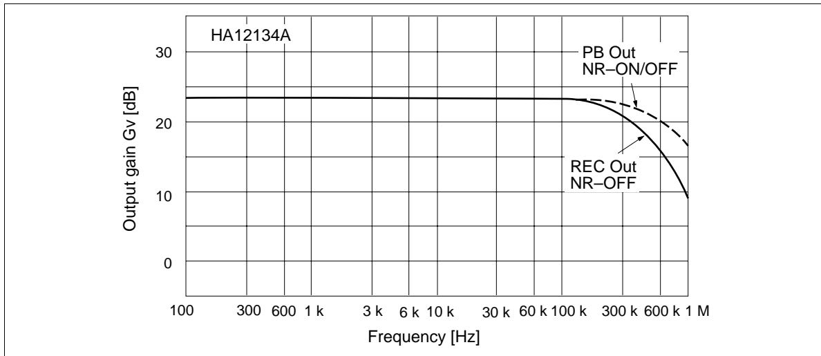
Figure 27 REC Mode Output Gain vs. Frequency
