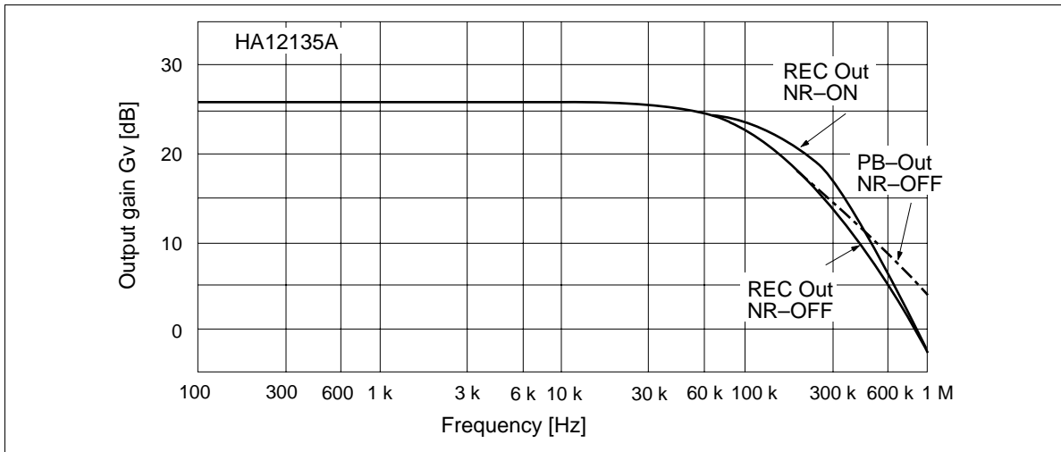
Figure 17 PB Mode Output Gain vs. Frequency
