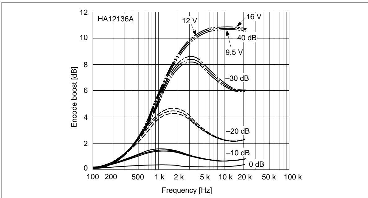
Figure 4 Encode Boost vs. Frequency
