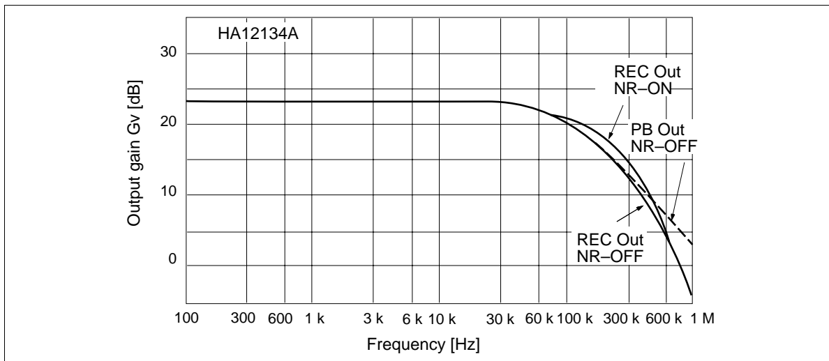
Figure 28 PB Mode Output Gain vs. Frequency
