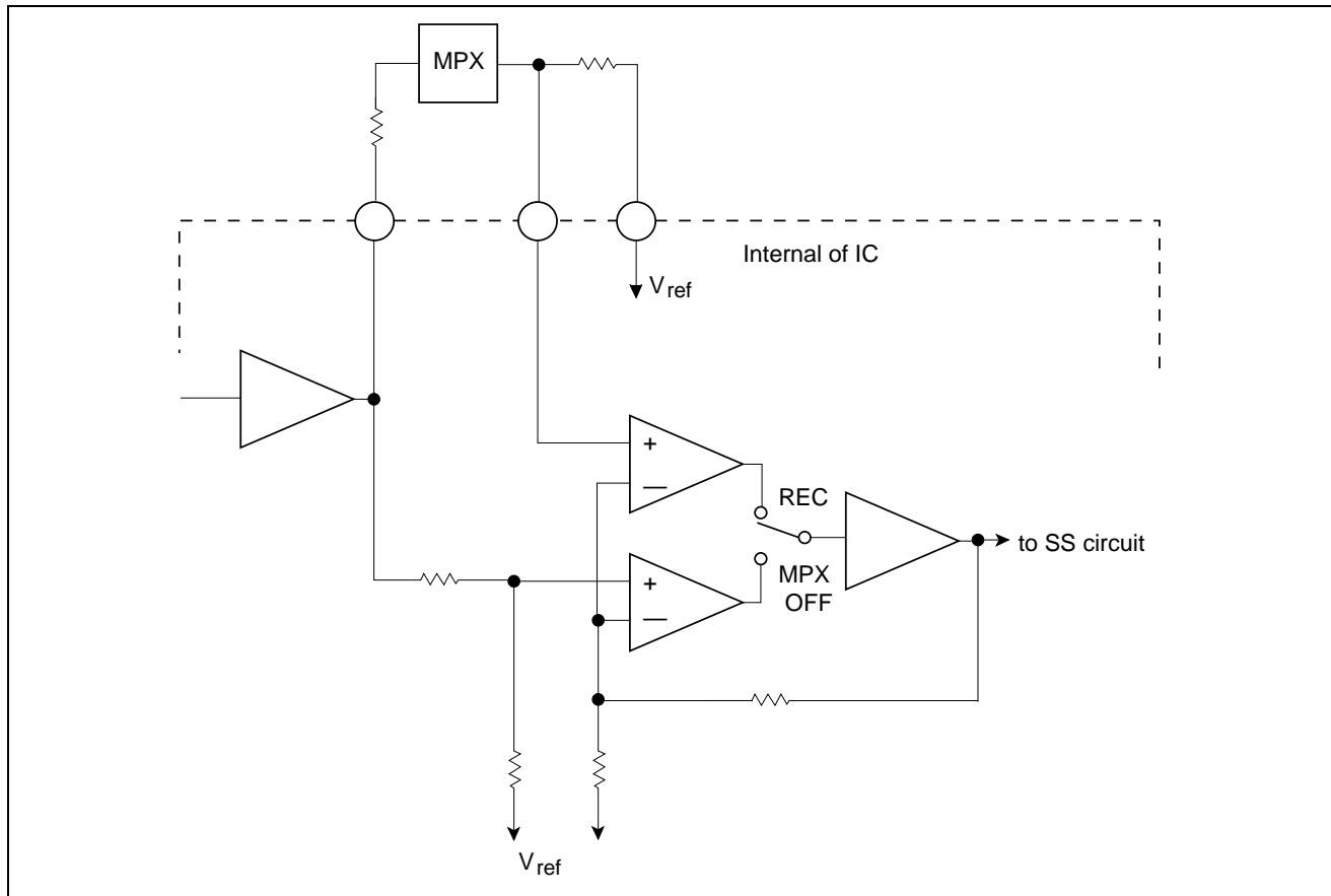
Figure 2 The Block-Diagram of MPX Driving Circuit
