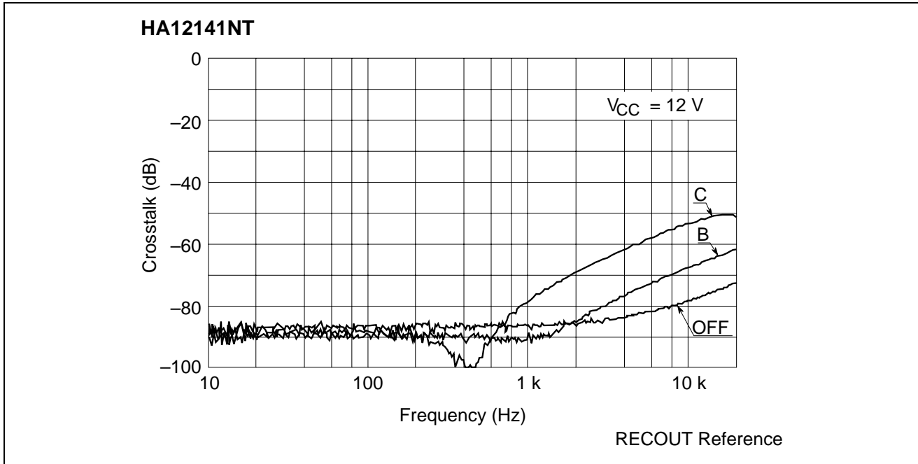
Crosstalk vs. Frequency (REC MODE R→L)
