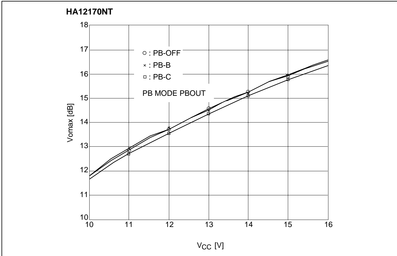
Maximum Output Level vs. Supply Voltage
