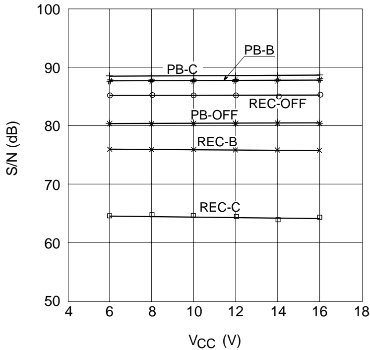
S/N vs. Supply Voltage
