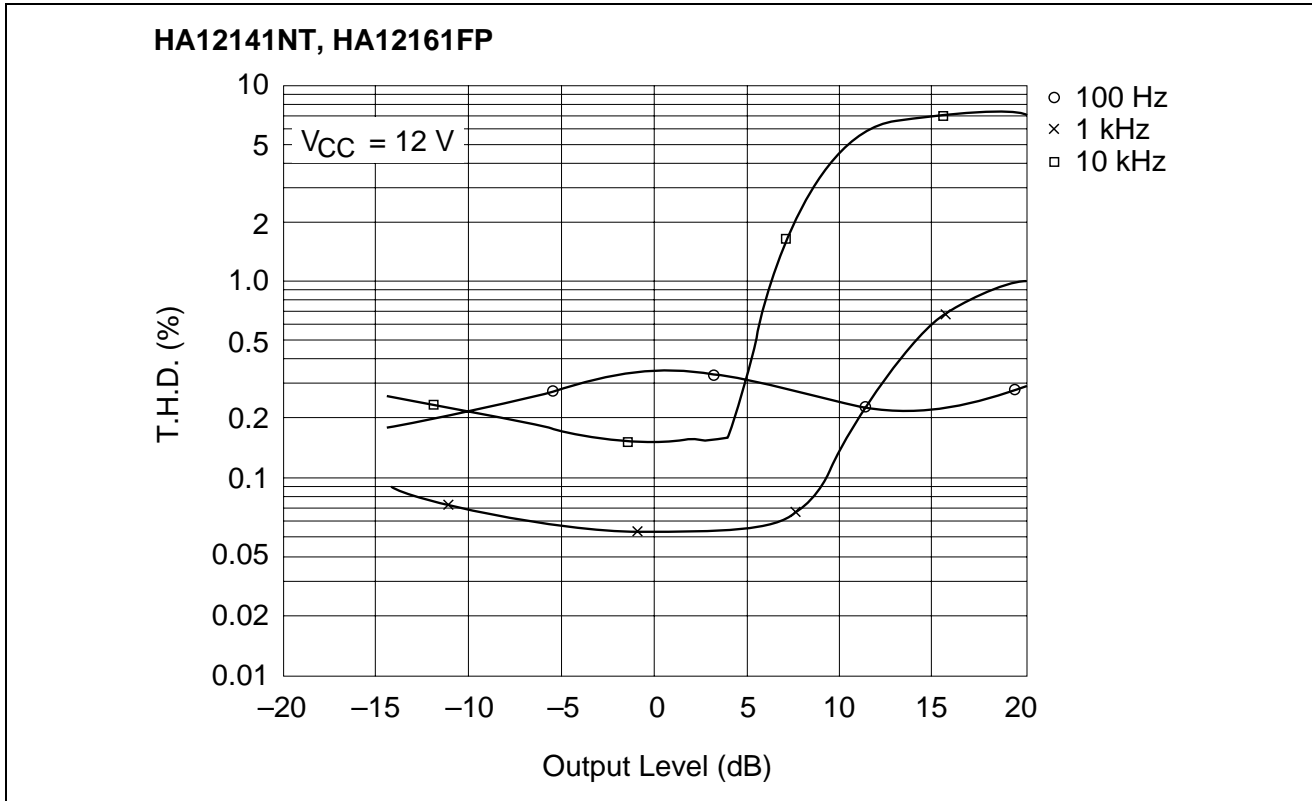
Total Harmonic Distortion vs. Output Level (PB MODE NR-C)
