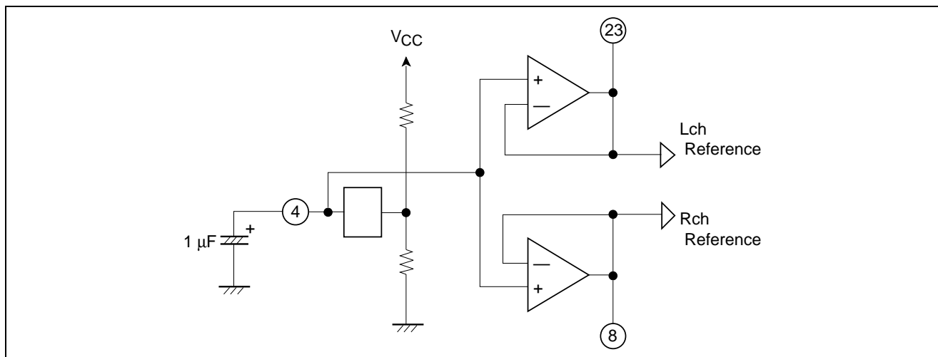
Figure 1 The Block-Diagram of Reference Voltage Supply
