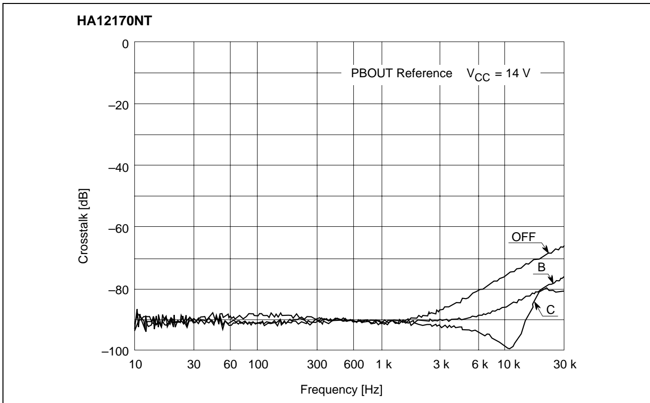
Crosstalk vs. Frequency (PB MODE R↔L)
