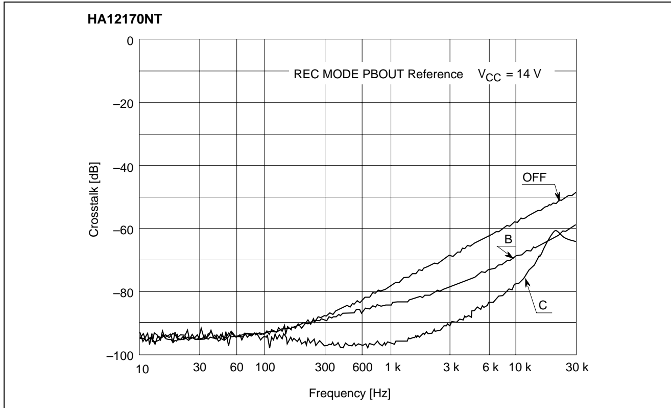
Crosstalk vs. Frequency (REC→PB)
