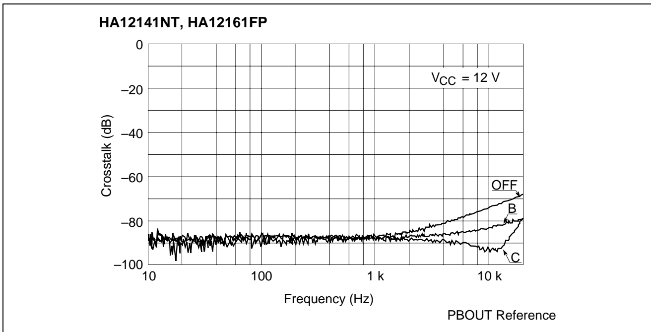
Crosstalk vs. Frequency (PB MODE R→L)
