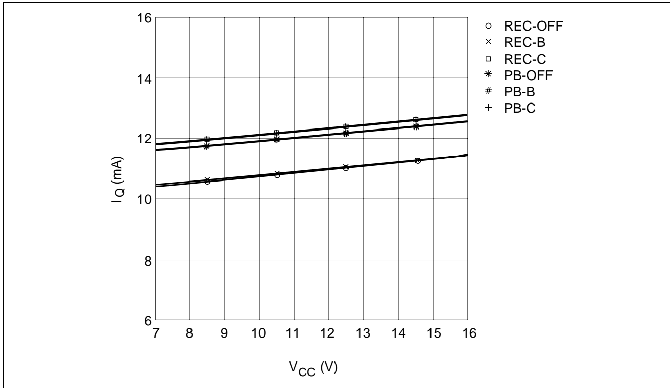
Quiescent Circuit vs. Supply Voltage
