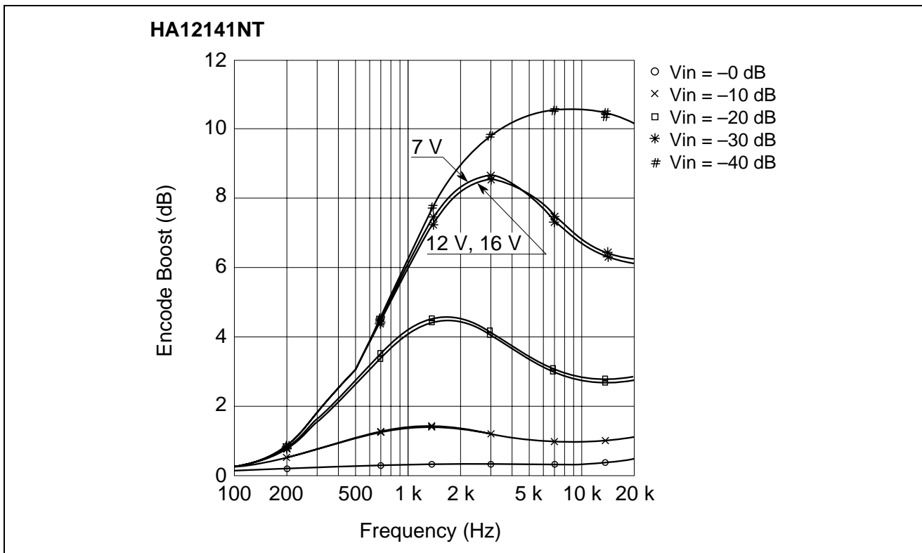
Encode Boost vs. Frequency (NR-B V_{CC} = 7V, 12 V, 16 V )
