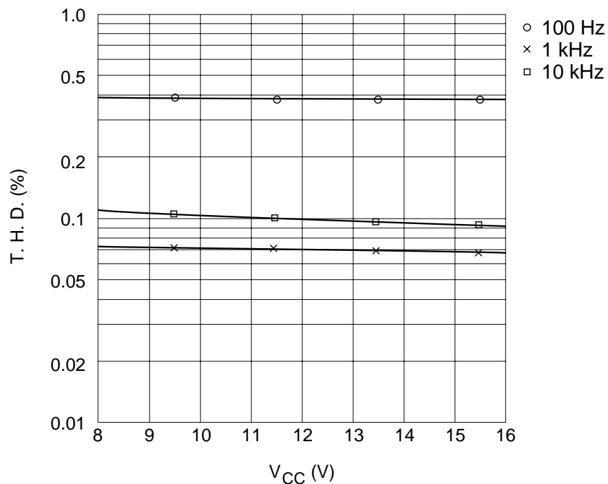
Total Harmonic Distortion vs. Supply Voltage (REC MODE NR-C)
