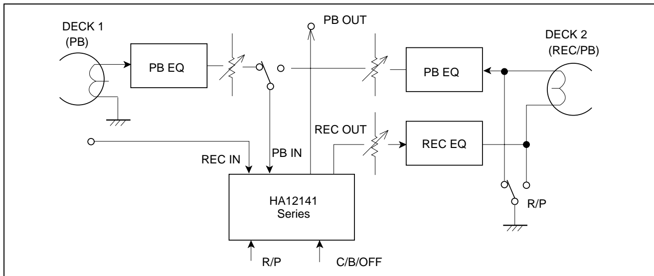
Figure 5 Application for Dubbing Deck
