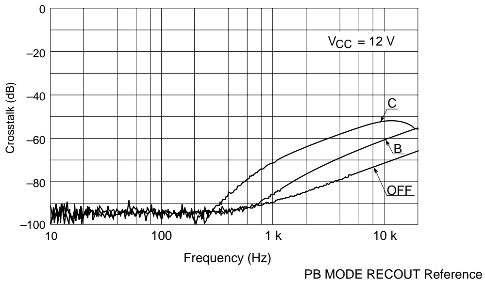
Crosstalk vs. Frequency (PB→REC)
