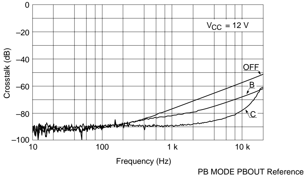
HA12141NT, HA12161FP
