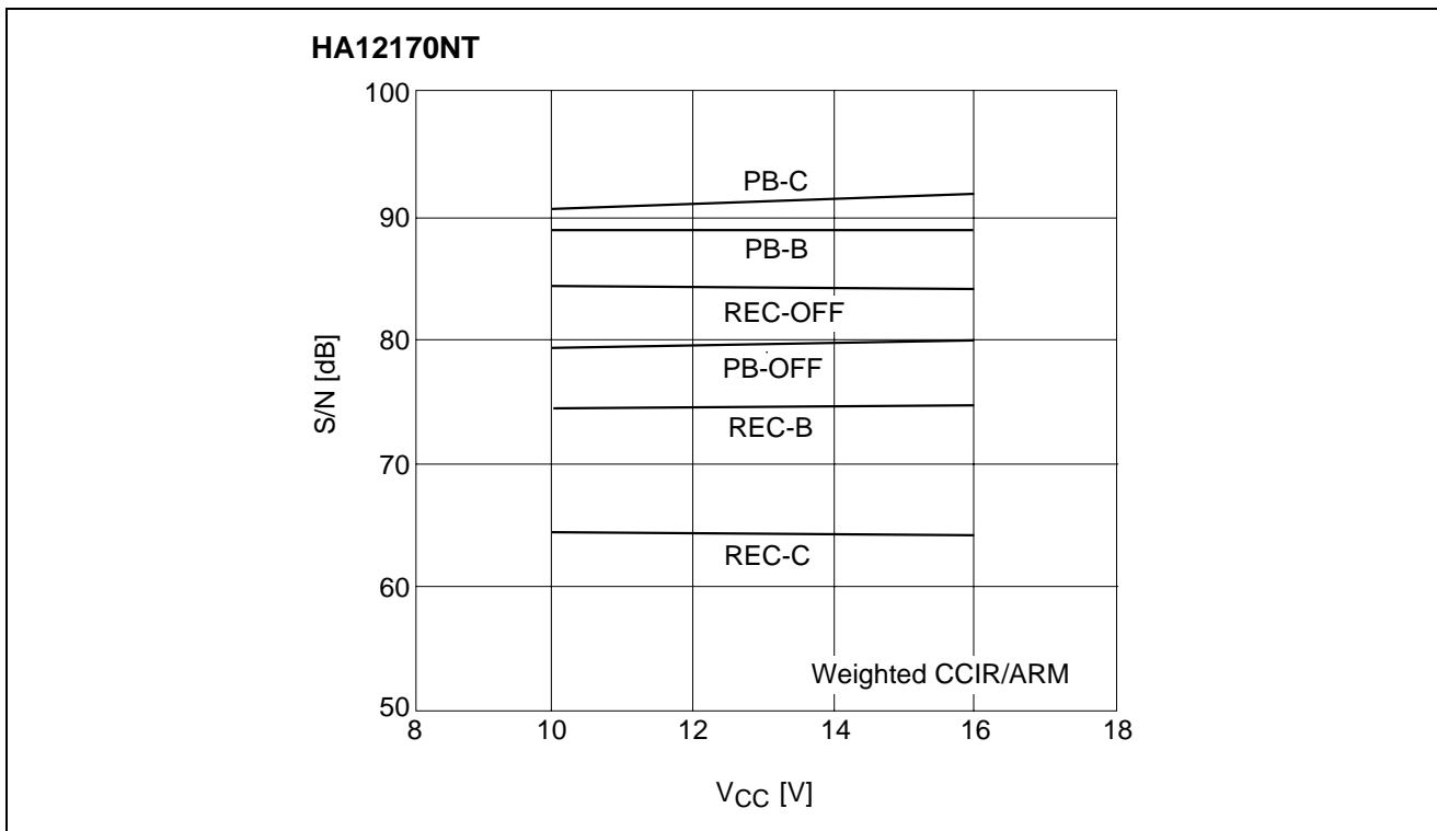
S/N vs. Supply Voltage
