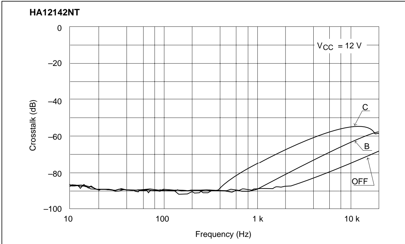
Crosstalk vs. Frequency (PB→REC)
