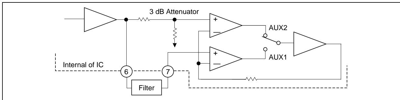
Figure 4 Application of AUX Mode
