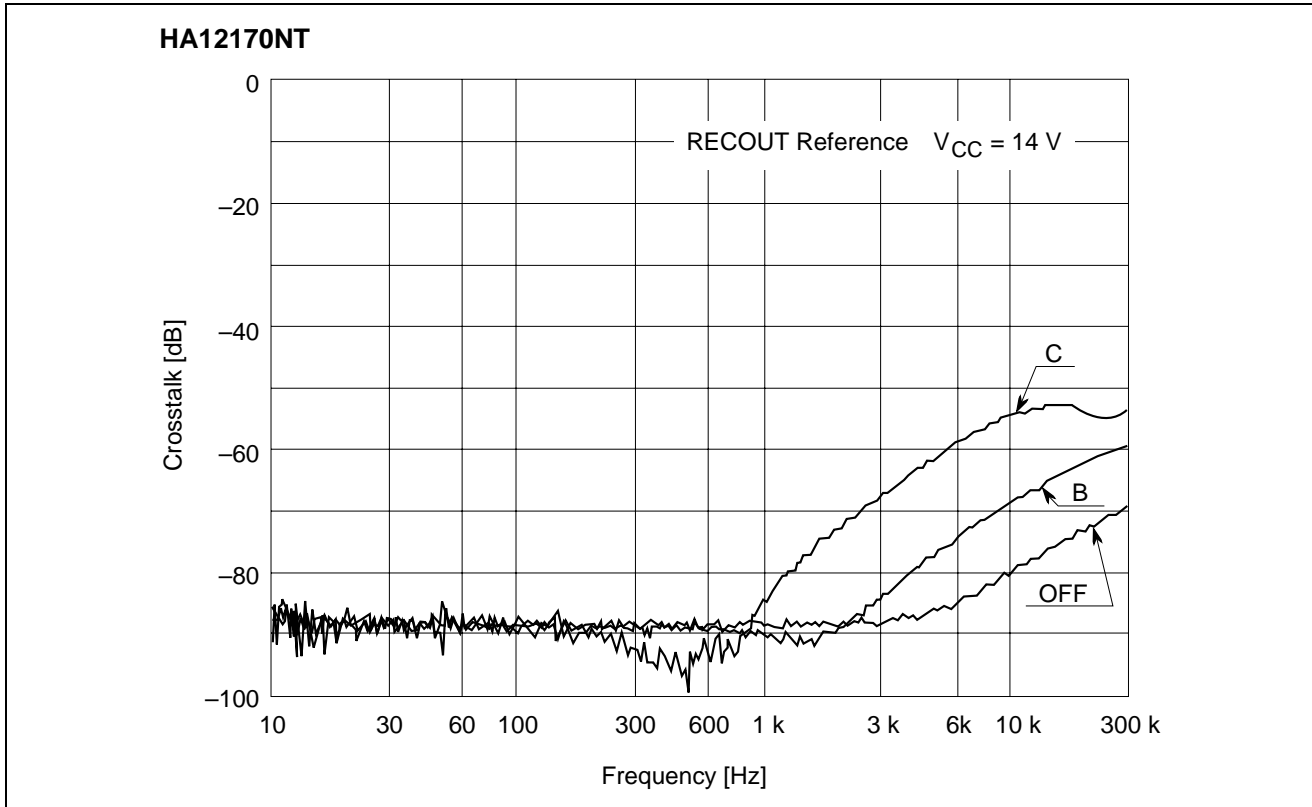
Crosstalk vs. Frequency (REC MODE R↔L)
