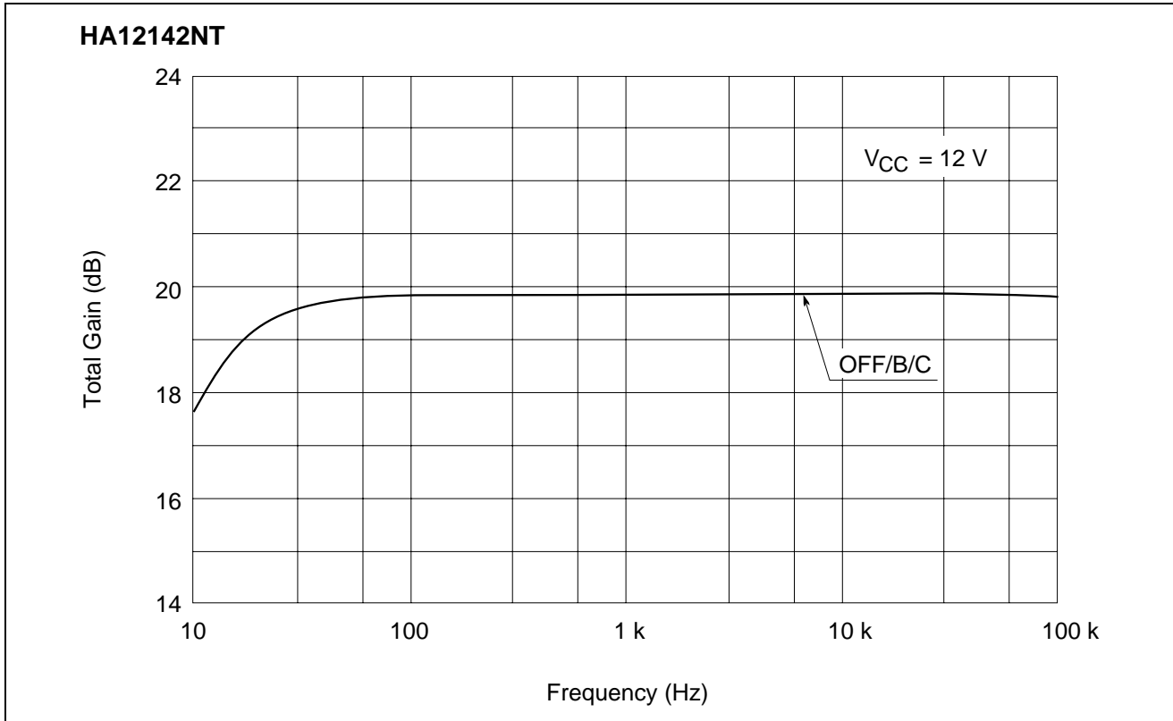
Total Gain vs. Frequency (PB MODE RECOUT)
