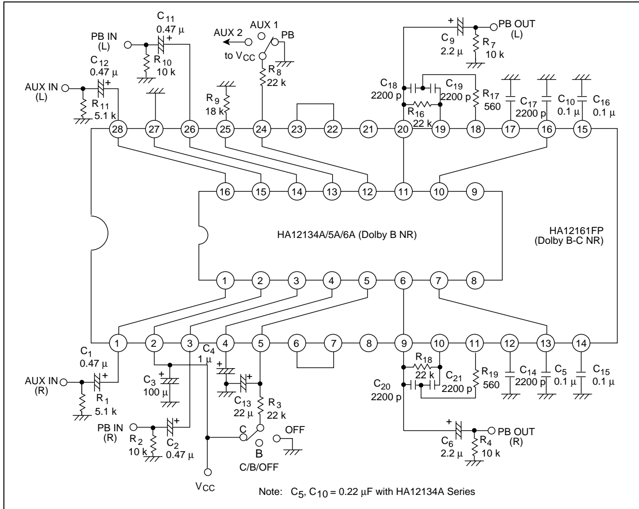
Figure 3 Application of HA12161FP/162FP
