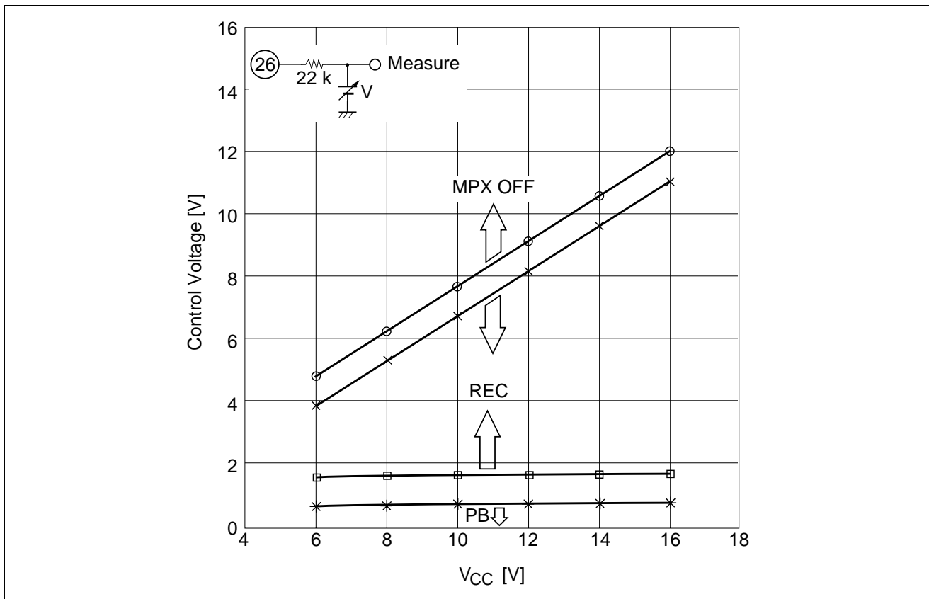
Control Voltage vs. Supply Voltage (PB/REC/MPX)
