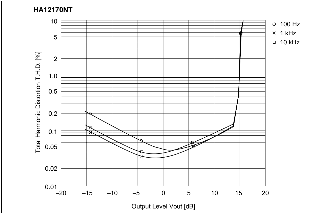
Total Harmonic Distortion vs. Output Level (REC MODE NR-OFF V_{cc} = 14\text{ V} )
