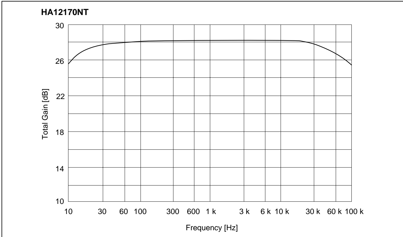
Total Gain vs. Frequency (PB MODE PBOUT NR-OFF V_{cc} = 14\text{ V} )
