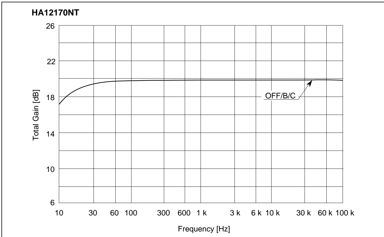
Total Gain vs. Frequency (PB MODE RECOUT V_{cc} = 14 V )
