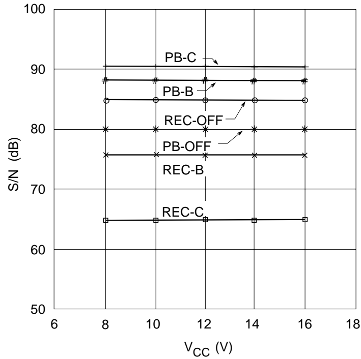
HA12142NT, HA12162FP
