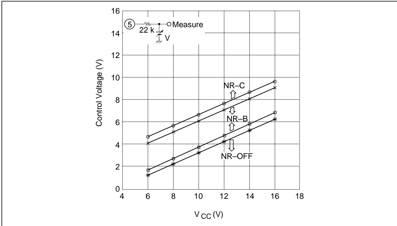
Control Voltage vs. Supply voltage (NR-OFF/B/C)
