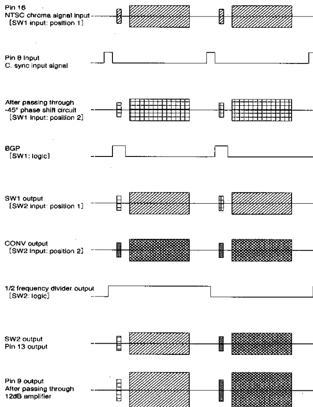
Fig.1 Timing chart
