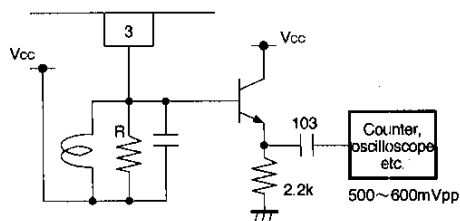
Fig. 4 Tank circuit
