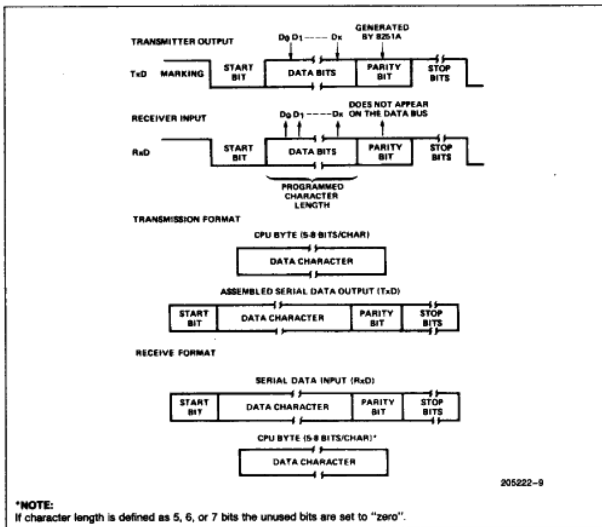
Figure 9. Asynchronous Mode
