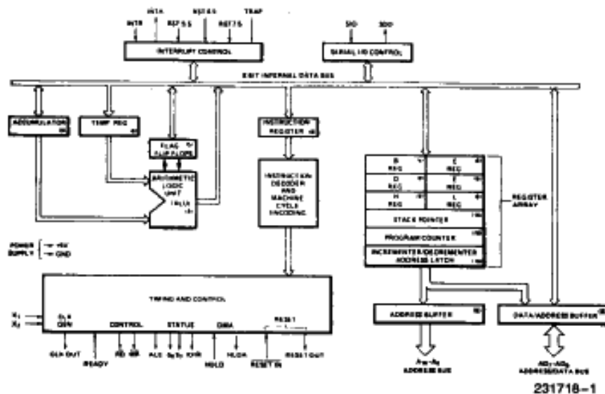
Figure 1. 8085AH CPU Functional Block Diagram
