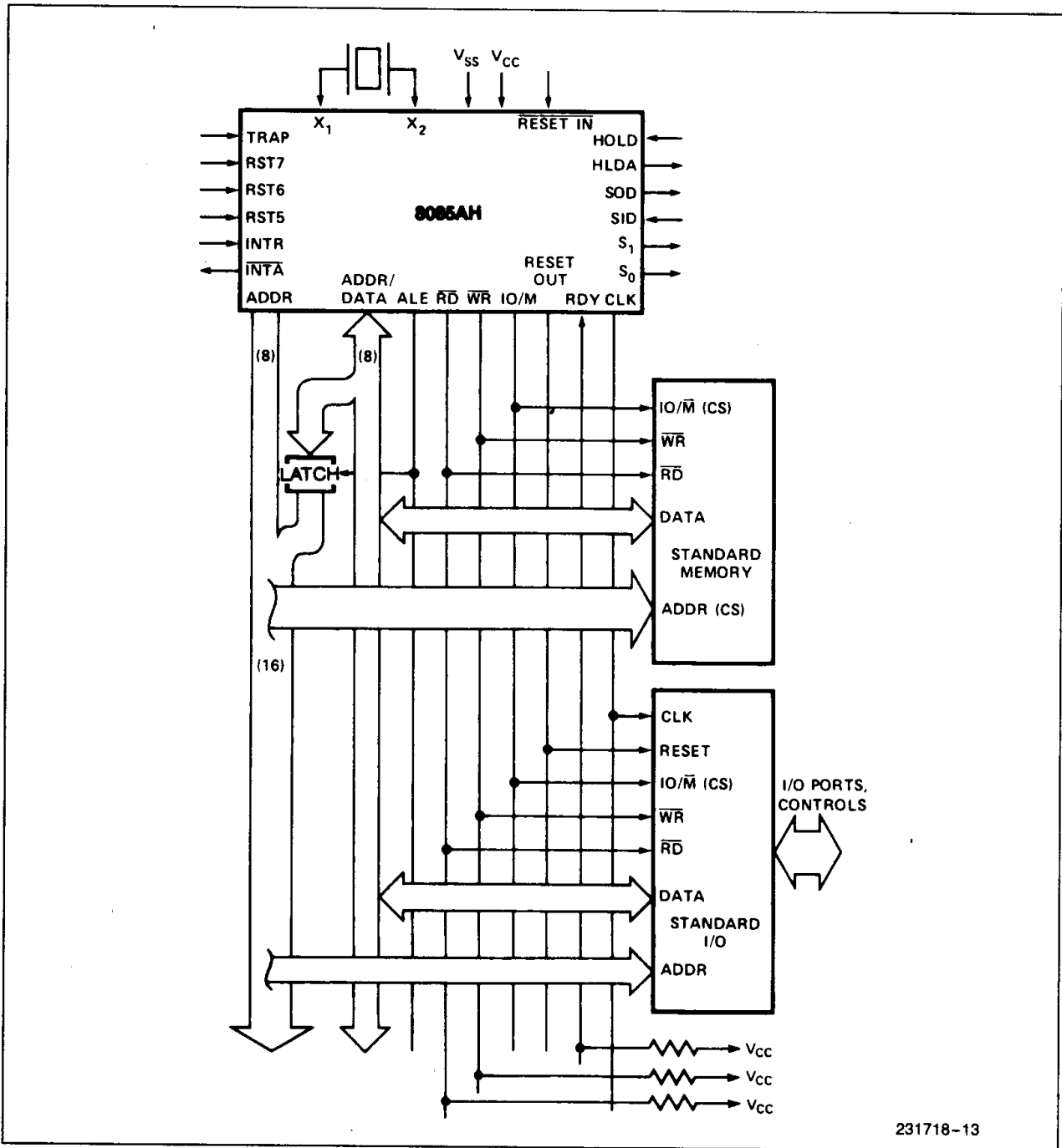
Figure 9. 8085 System (Using Standard Memories)
