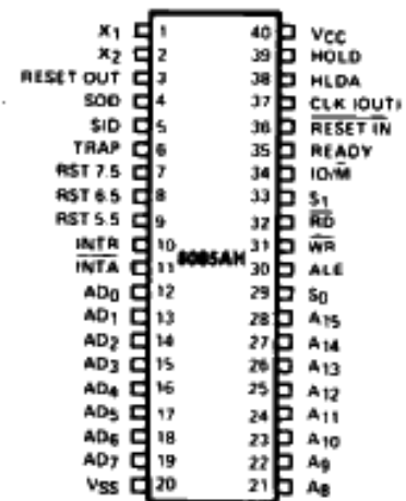
Figure 2. 8085AH Pin Configuration
