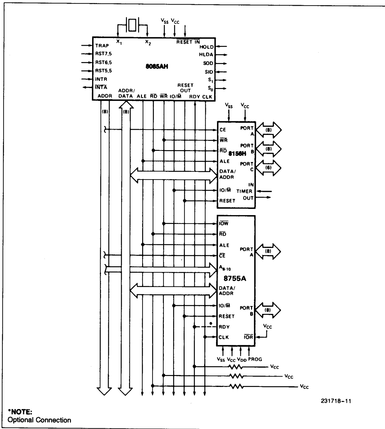
Figure 7. 8085AH Minimum System (Standard I/O Technique)
