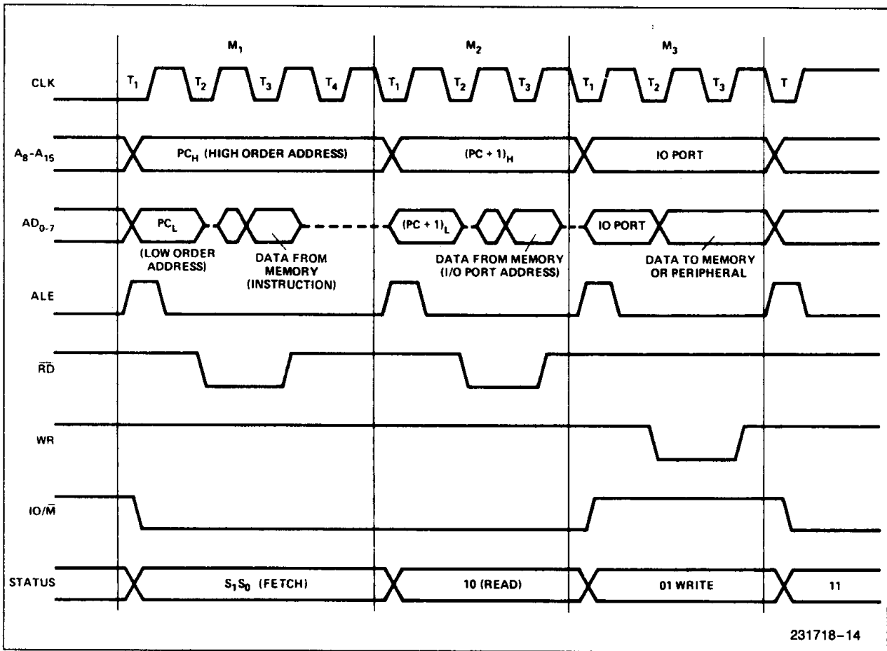
Figure 10. 8085AH Basic System Timing
