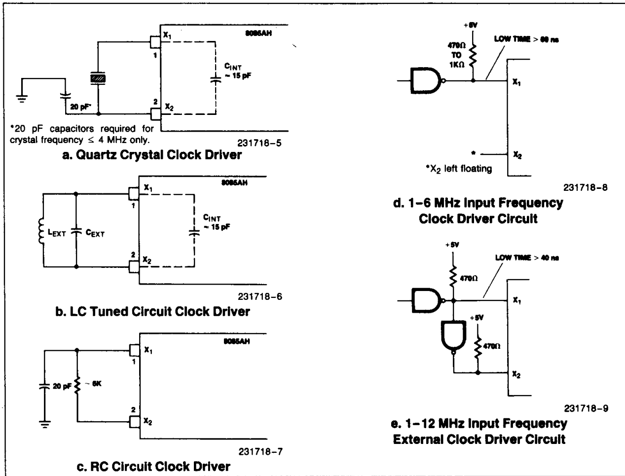
Figure 5. Clock Driver Circuits
