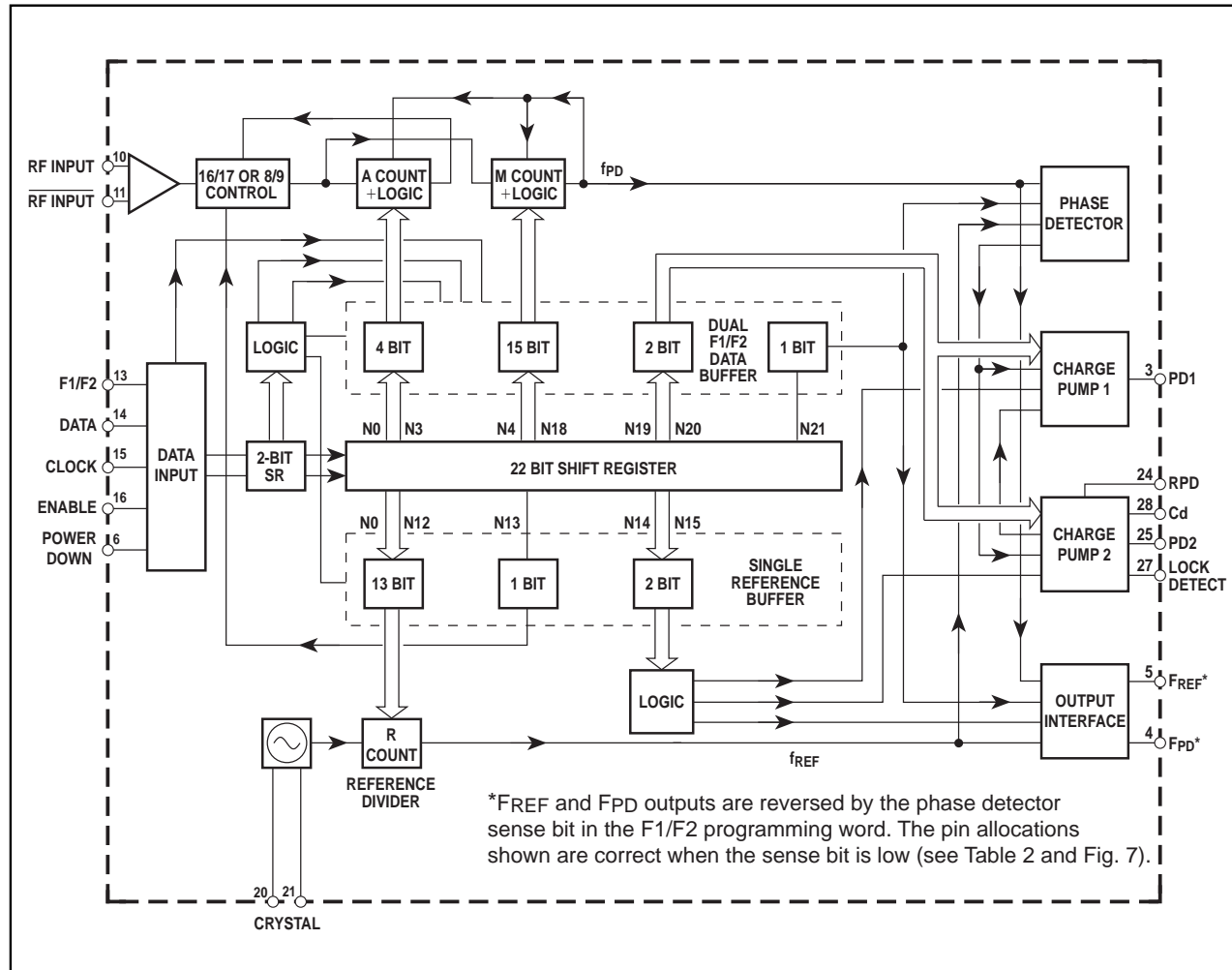
Fig. 2 SP8853 block diagram
