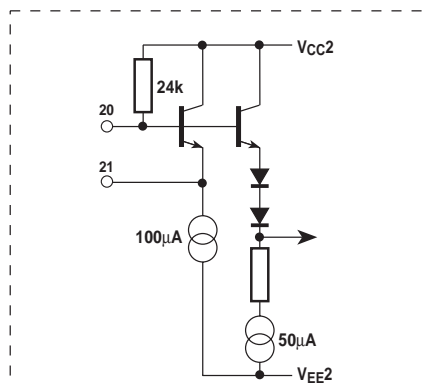
Fig. 8d Oscillator pins
