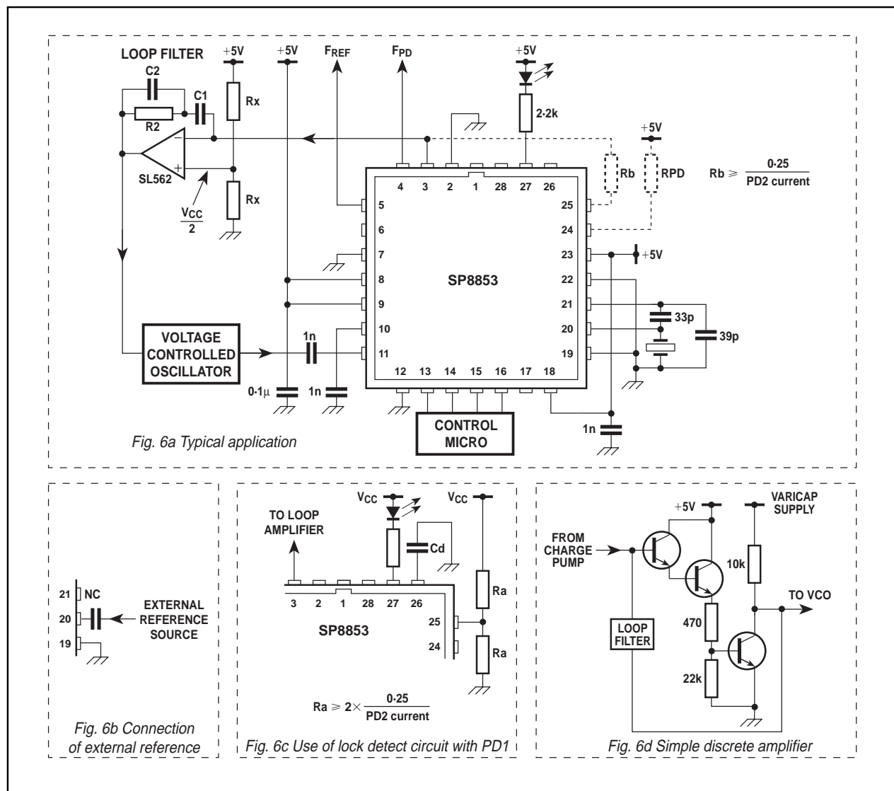
Fig. 6 Application diagrams
