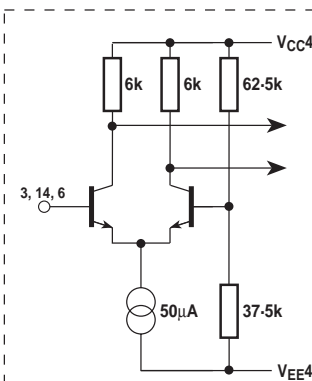
Fig. 8b F1/F2 data and power down inputs
