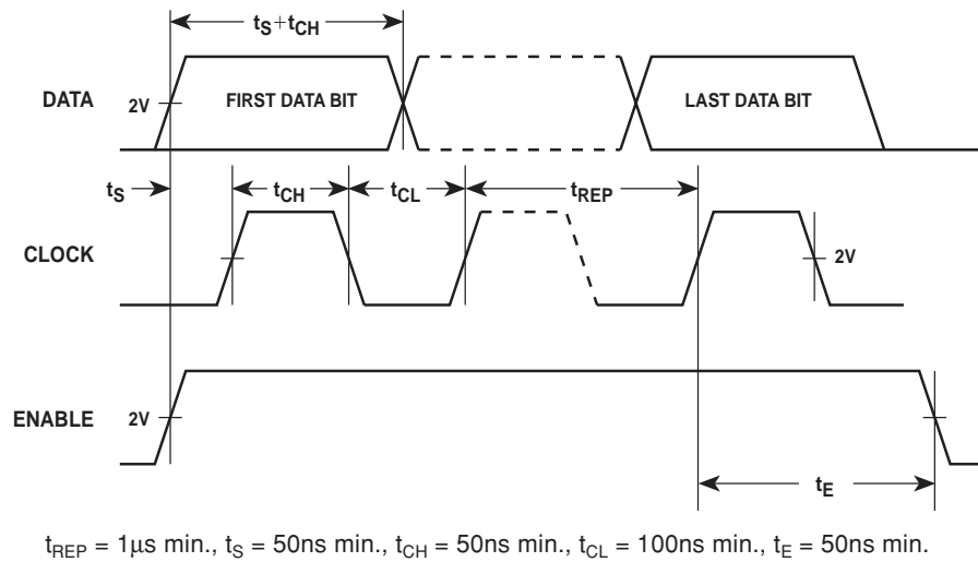
Fig. 5 Data and clock timing requirements
