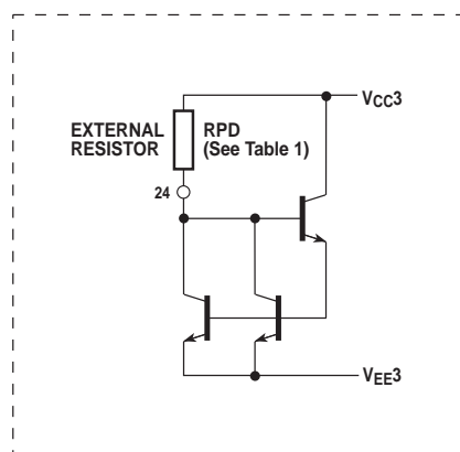
Fig. 8g Charge pump 2 current programming
