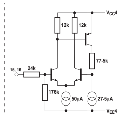
Fig. 8c Hysteresis inputs, data clock and enable
