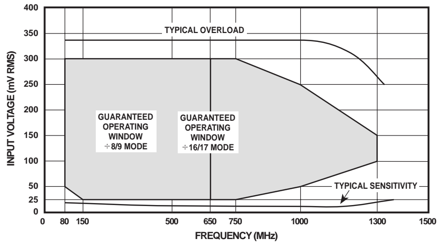
Fig. 4 Typical input characteristics and input drive requirements for SP8853 A and B
