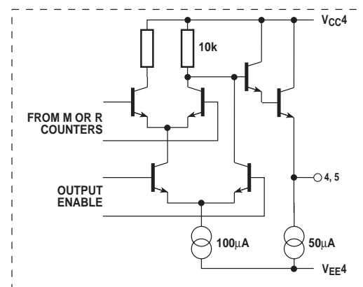
Fig. 8h FPD and FREF outputs
