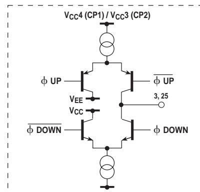
Fig. 8f Phase detector charge pumps
