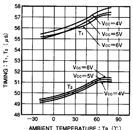
Fig. 15 One-shot timing period vs. ambient temperature characteristic
