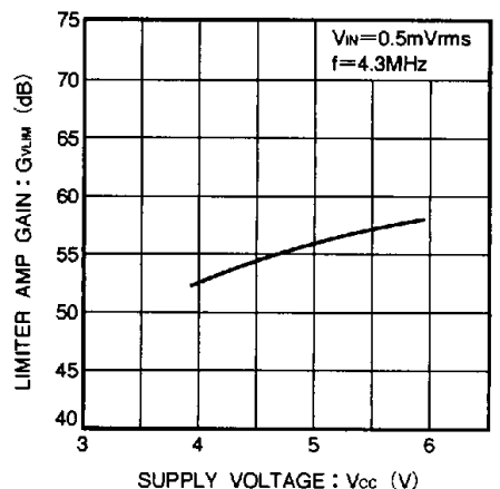
Fig. 12 Limiter amplifier gain vs. supply voltage characteristic
