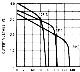
Output High Voltage (Logical "1") vs Output Current
