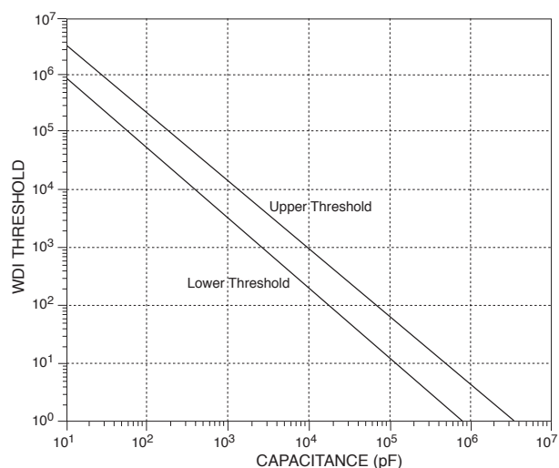
Watchdog Frequency Threshold vs C_{DELAY}
