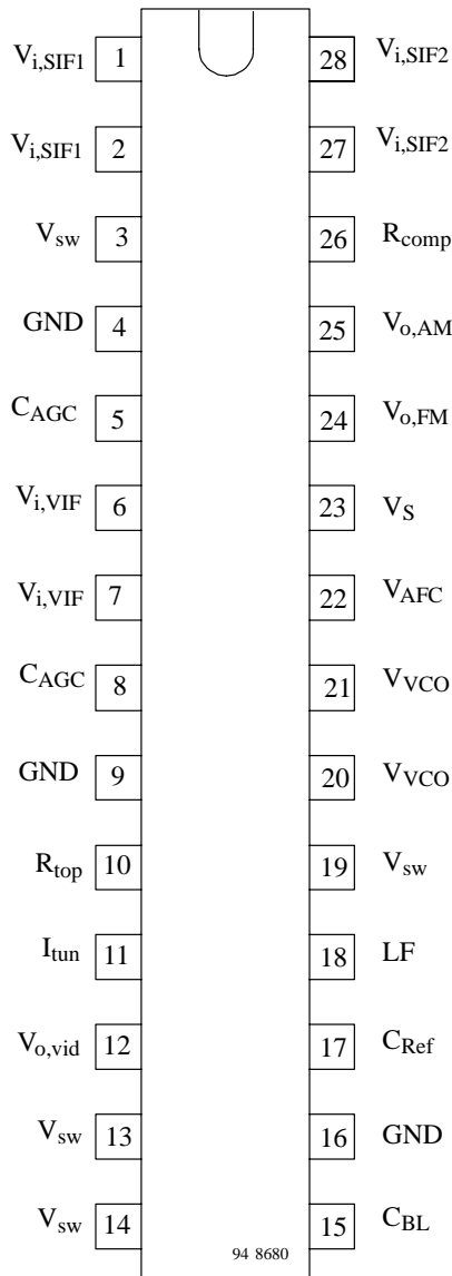
Figure 2. Pinning
