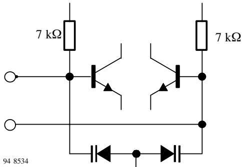
Figure 18. VCO (Pin 20-21)
