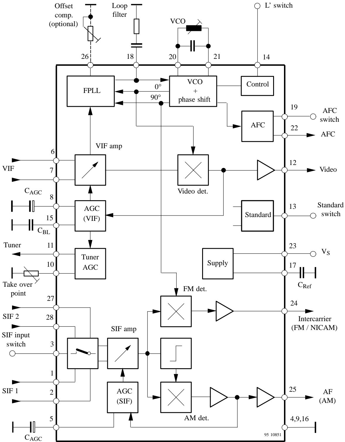
Figure 1. Block diagram
