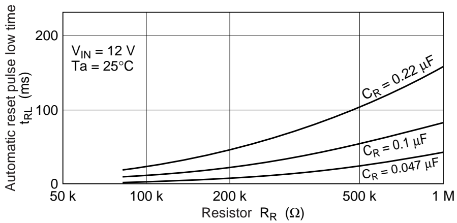
Figure 5 Automatic Reset Pulse Low Time vs. Resistor
