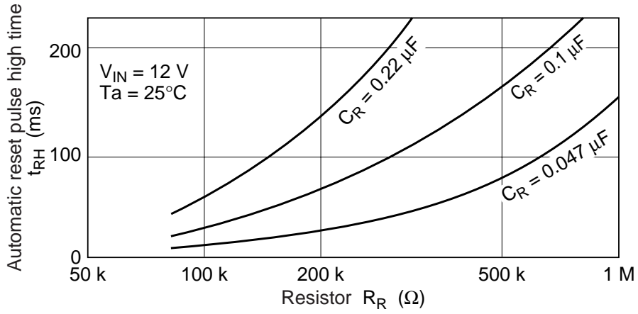
Figure 4 Automatic Reset Pulse High Time vs. Resistor
