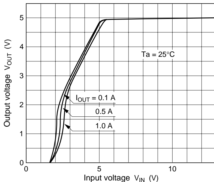
Figure 1 Output Voltage vs. Input Voltage
