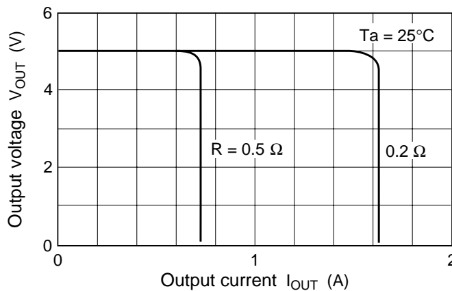
Figure 2 Output Voltage vs. Output Current
