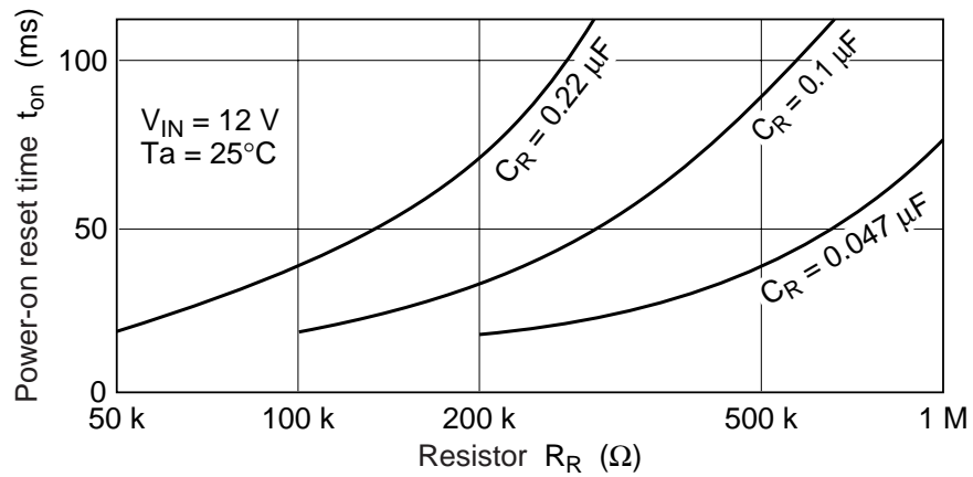
Figure 6 Power-on Reset Time vs. Resistor
