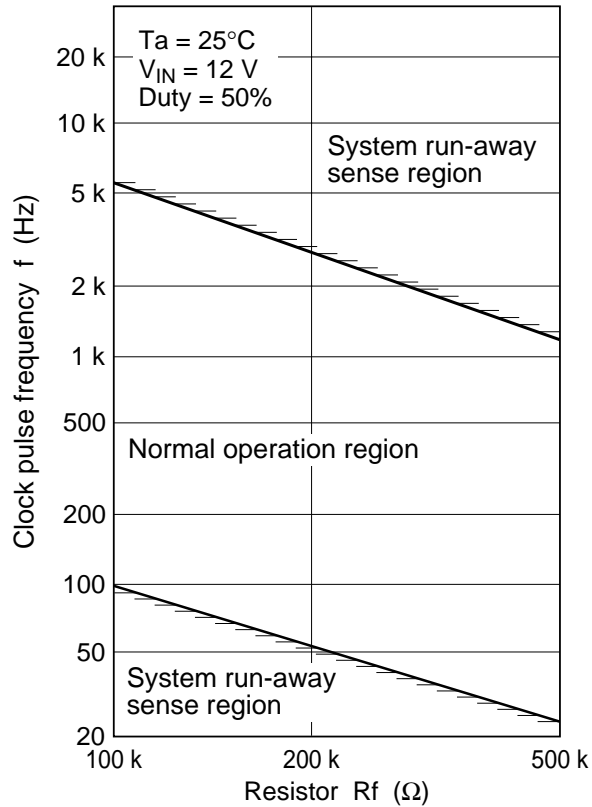
Figure 8 Clock Pulse Frequency vs. Resistor
