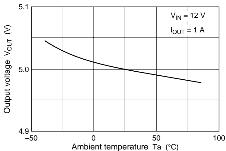
Figure 3 Output Voltage vs. Ambient Temperature
