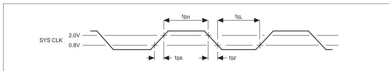
Figure 7: Timing - system clock
