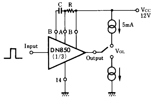
Test Circuit 2 ( f , V_{OH} , V_{OL} )
