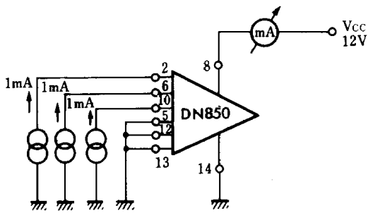
Test Circuit 3 ( I_{CCH} )
