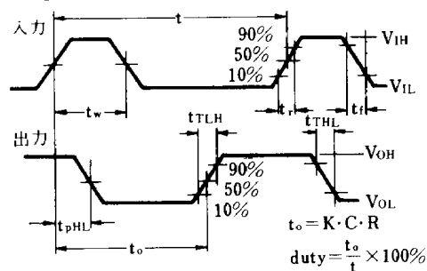
*1 Timing Diagram
