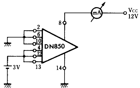
Test Circuit 4 ( I_{CCL} )
