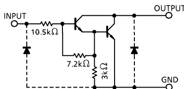
TD62104P / F
