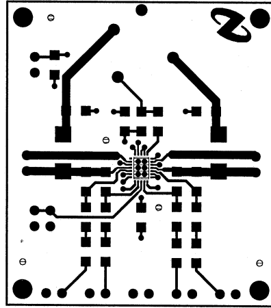
10099340 Figure 8. Recommended LQ PC Board Layout: Component-Side Layout
