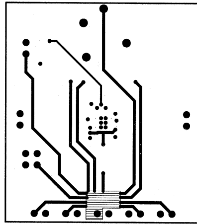
10099342 Figure 10. Recommended LQ PC Board Layout: Lower Inner-Layer Layout
