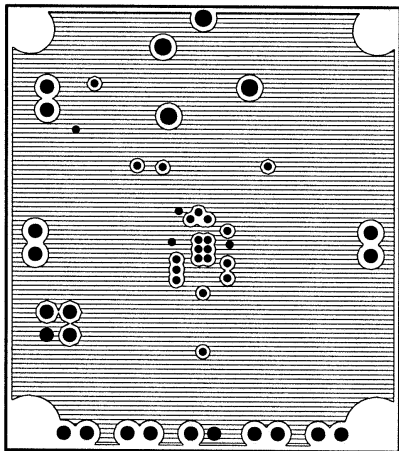
10099341 Figure 9. Recommended LQ PC Board Layout: Upper Inner-Layer Layout
