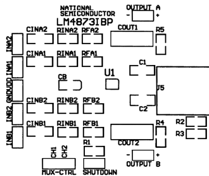
10099344 Figure 12. Recommended 20-pin micro SMD PC Board Layout: Component-Side Silkscreen
