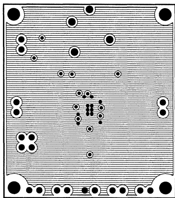
10099343 Figure 11. Recommended LQ PC Board Layout: Bottom-Side Layout
