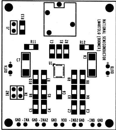
10099339 Figure 7. Recommended LQ PC Board Layout: Component-Side Silkscreen
