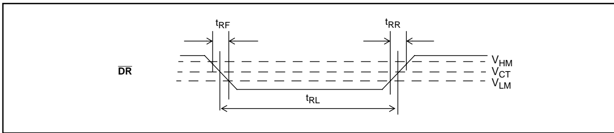
Figure 11 - DR Output Timing
