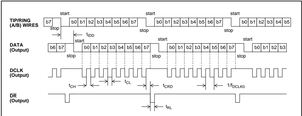
Figure 13 - Serial Data Interface Timing (Mode 0)
