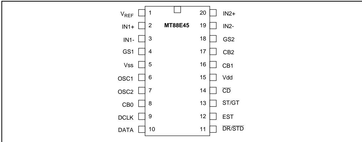
Figure 2 - Pin Connections
