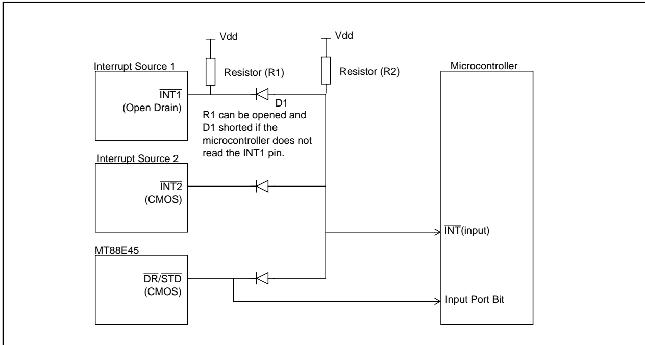
Figure 9 - Application Circuit: Multiple Interrupt Source
