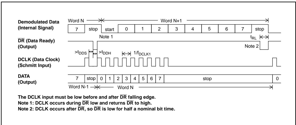
Figure 14 - Serial Data Interface Timing (Mode 1)
