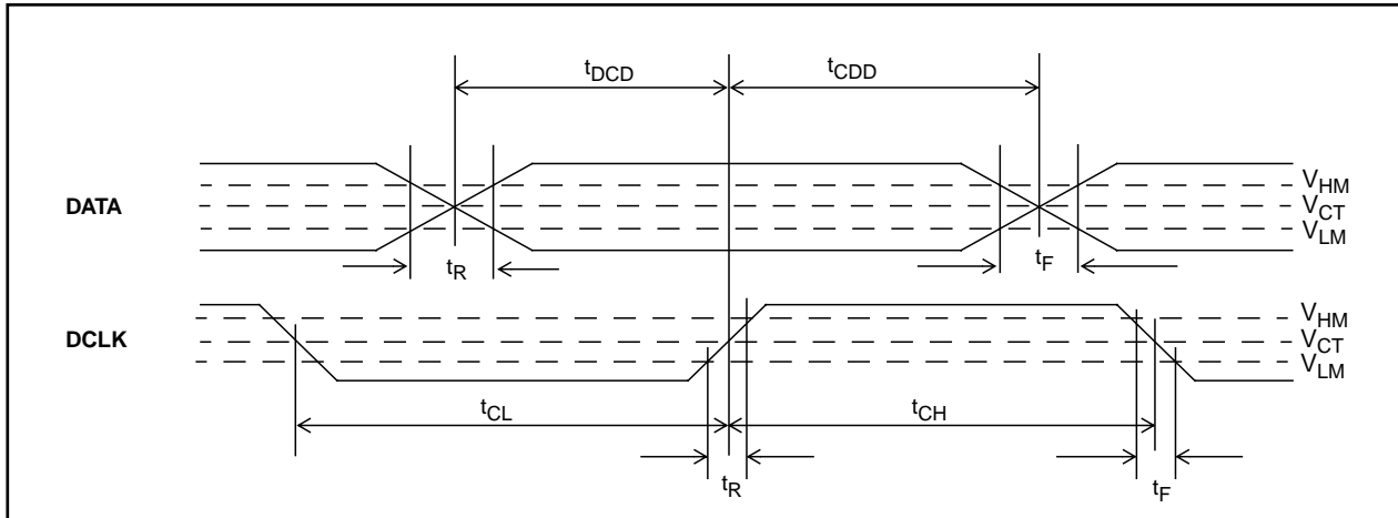
Figure 10 - DATA and DCLK Mode 0 Output Timing
