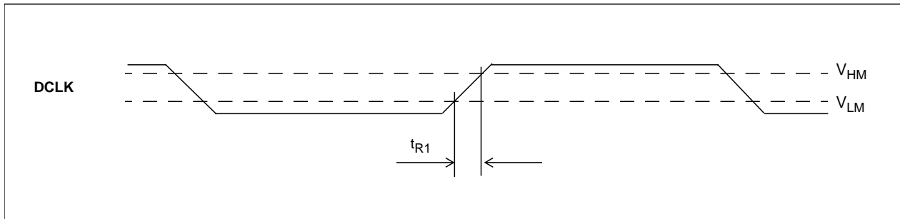
Figure 12 - DCLK Mode 1 Input Timing
