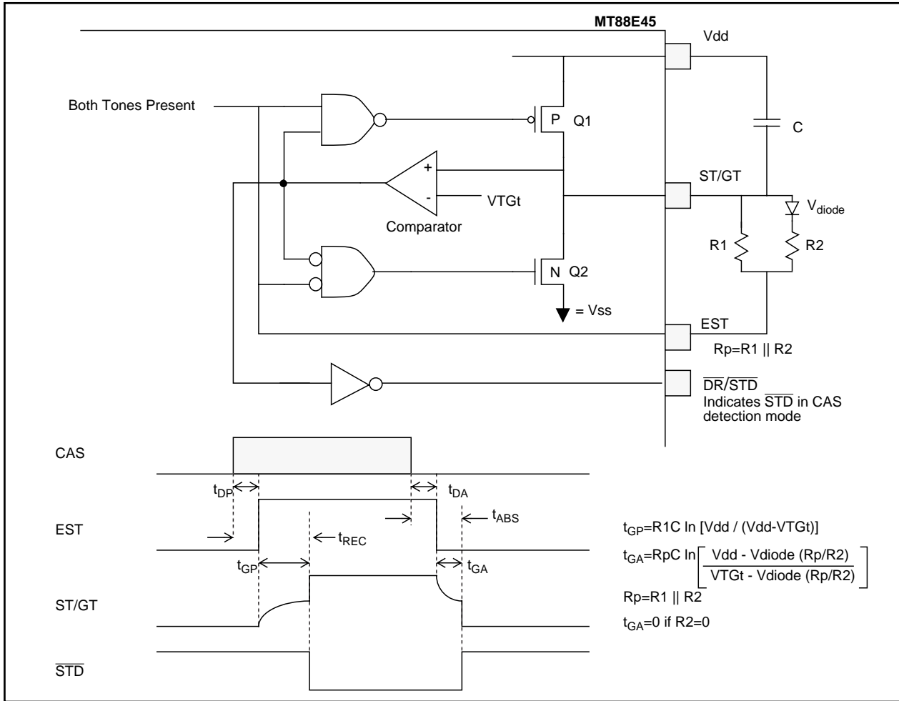
Figure 5 - CAS Guard Time Circuit Operation
