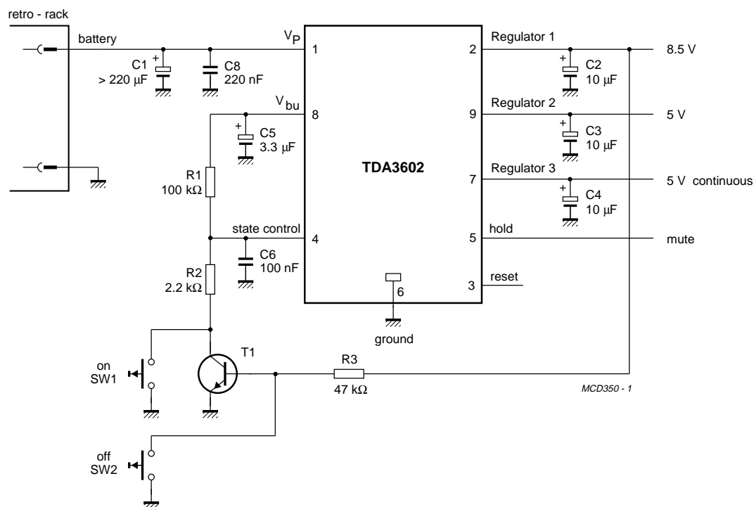
Fig.8 Application circuit 2.
