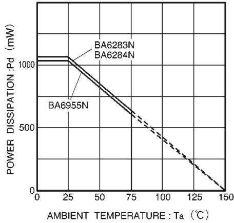
Fig.6 Package thermal derating characteristics
