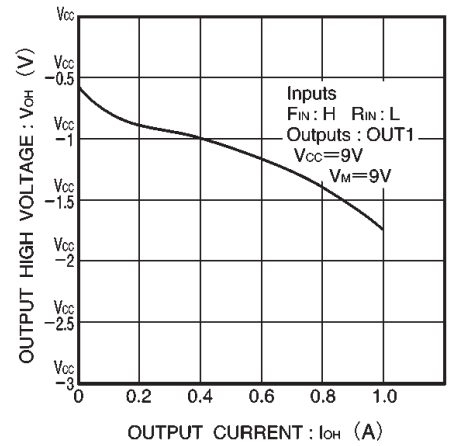
Fig.8 Output high level voltage vs. output current
