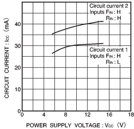
Fig.7 Circuit current vs. power supply voltage
