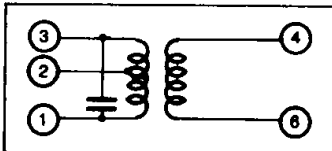
T2 AM IFT (MIX OUT)
