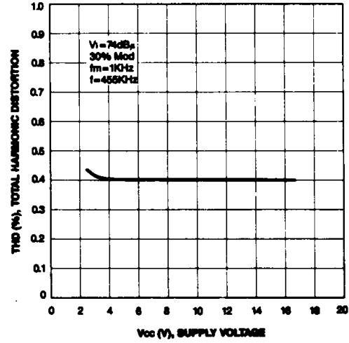
TOTAL HARMONIC DISTORTION-SUPPLY VOLTAGE
