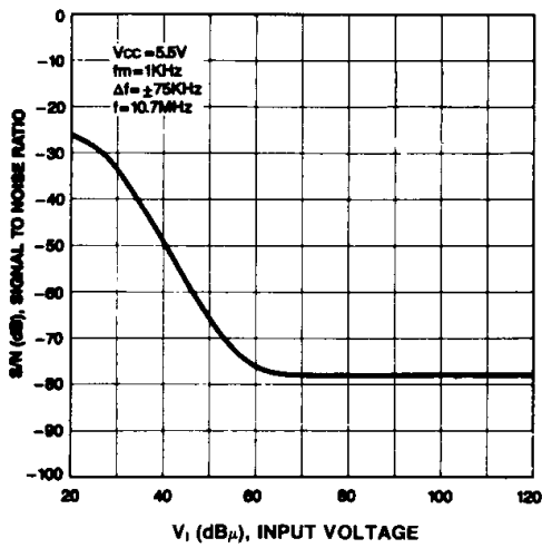
SIGNAL TO NOISE RATIO-INPUT VOLTAGE
