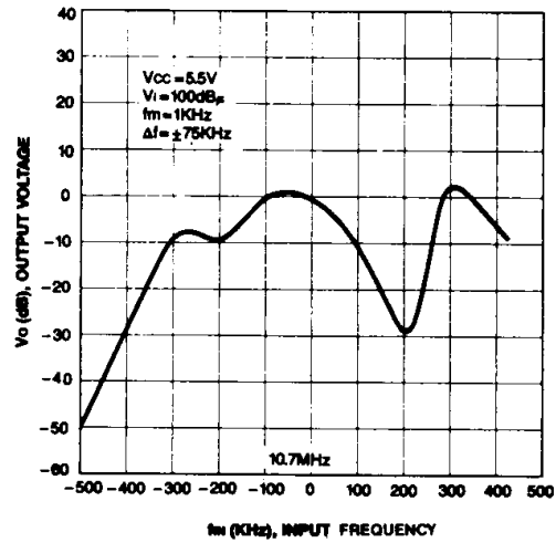
OUTPUT VOLTAGE-INPUT FREQUENCY
