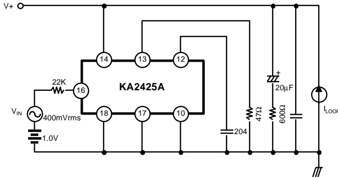
Fig 2. DTMF Driver Test
