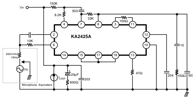
Fig 3. Transmit and sidetone level test
