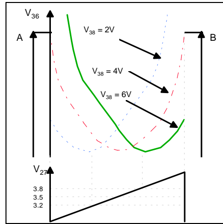
Figure 2. Keystone Adjustment
