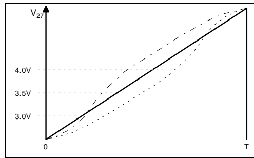
Figure 3. Amplitude Adjustment
