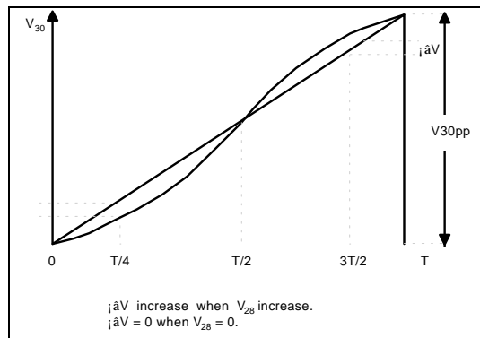
Figure 4. Correction Adjustment
