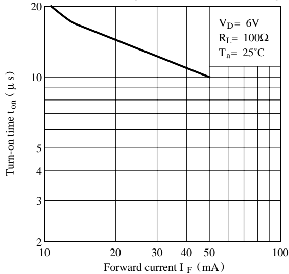
Fig.11 Turn-on Time vs. Forward Current (S16MD02/S26MD02)
