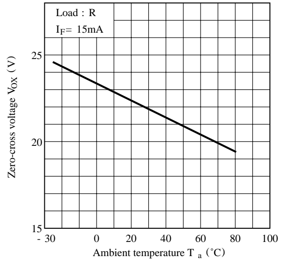
Fig.12 Zero-cross Voltage vs. Ambient Temperature (S16MD02/S26MD02)
