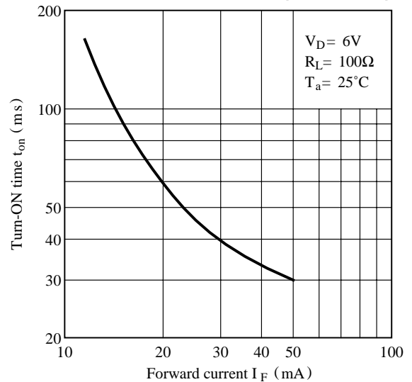
Fig.10 Turn-on Time vs. Forward Current (S26MD01)
