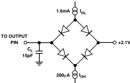
Figure 2. Load Circuit for Timing Specifications
