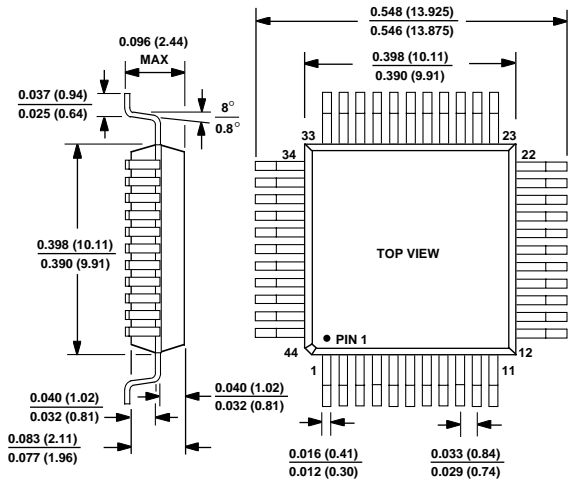
Plastic Quad Flatpack Package (S-44)
