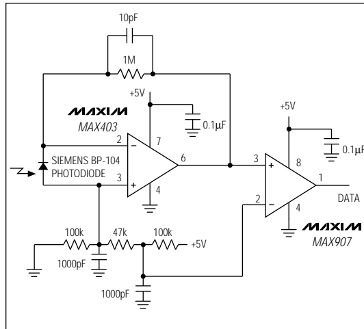
Figure 4. Battery-Operated Infrared Data Link Consumes Only 1mA
