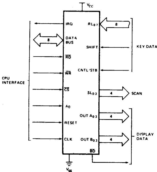
Figure 1. Logic Symbol
