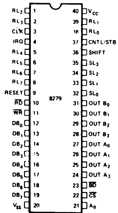
Figure 2. Pin Configuration
