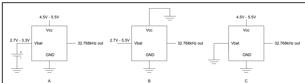
Figure 4. Power-Supply Connections
