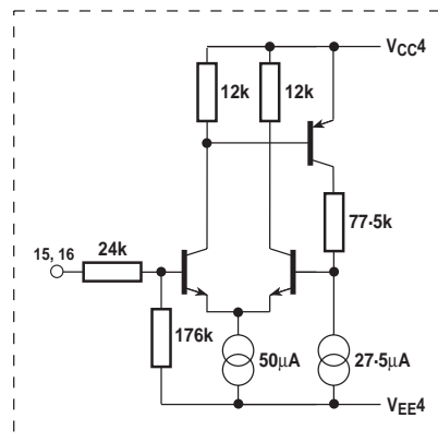
Fig. 8c Hysteresis inputs, data clock and enable
