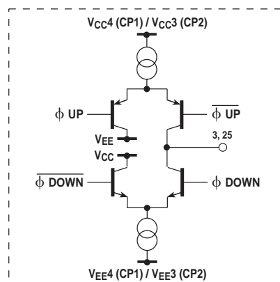
Fig. 8f Phase detector charge pumps
