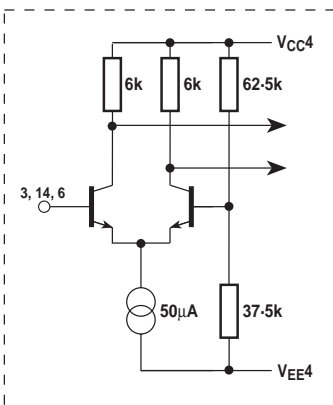
Fig. 8b F1/F2 data and power down inputs
