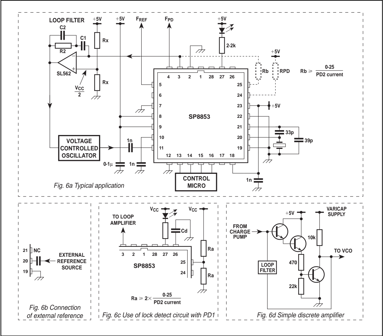
Fig. 6 Application diagrams
